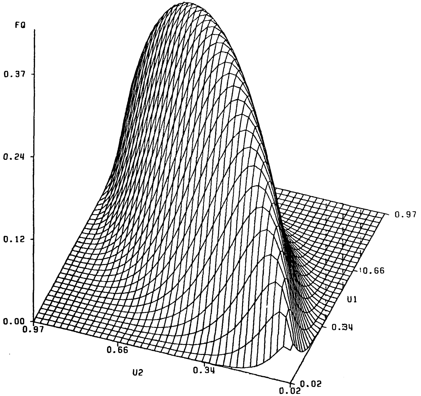
DENSITY-QUANTILE FOR BIVARIATE NORMAL CASE WITH RHO=0.9
