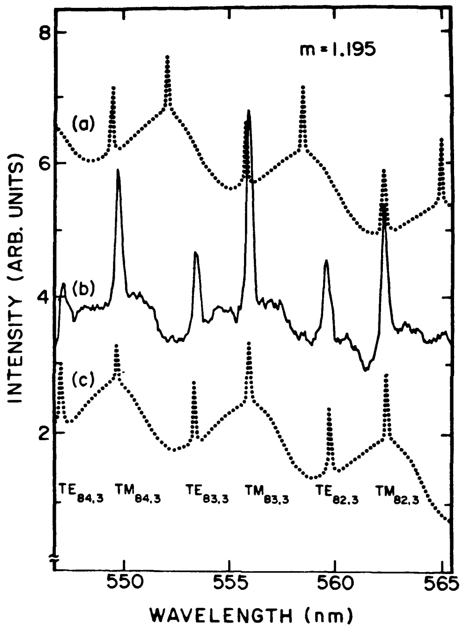
Figure 1. Fluorescence spectra from a single polystyrene sphere in water. In this wavelength range, the fluorescence spectra from a bulk medium is smooth. Curve a, theoretical result for a 9.92 \mu\text{m} sphere; curve b, the experimental result; and curve c, the theoretical result for a 9.99 \mu\text{m} sphere. The resonant peaks in curves b and c are identified by their mode numbers (84, 83, and 82) and mode orders (3).
