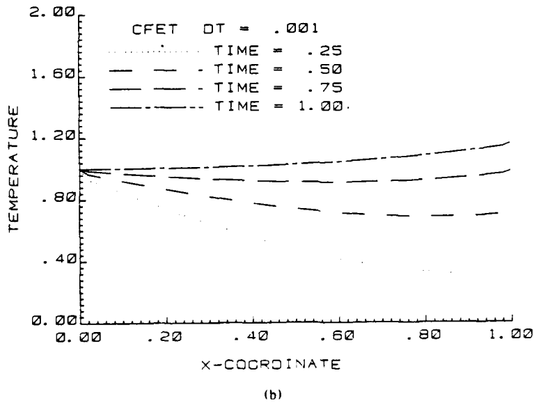
Fig. 30 — Temperature distribution ( V_0 = 0.0 , D_0 = 1.0 , Problem 7): (a) Displacement model and (b) Conventional model
