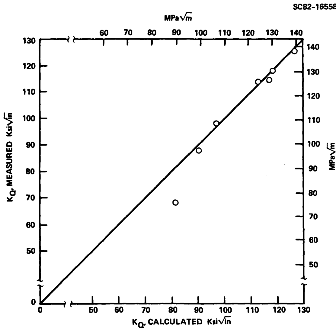
Fig. 17 Measured fracture toughness of solution treated Ti-4.5Al-5Mo-1.5Cr vs fracture toughness calculated using Eq. (3).
