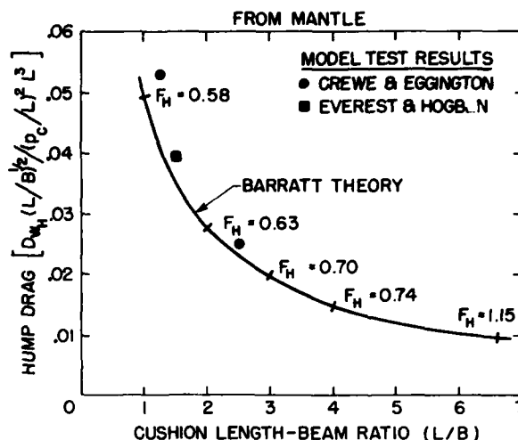
Fig. 2. Hump Wave Drag of ACV and SES, (Ref. 12)
