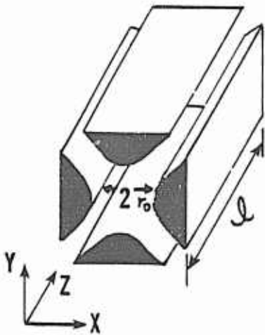
Figure 1. Electrode structure of the quadrupole and its relationship with the cartesian coordinate system. The coordinate system is oriented as shown but translated so that the origin is centered between the pole pieces as in figure 3. The ions, which move in a vacuum are introduced with a small velocity at x=0 , y=0 in the z direction. By imposing a voltage difference with DC and AC components on adjacent electrodes the device is tuned so that only ions with the proper mass to charge ratio traverse the length of the filter where they are detected. Ions with a different mass to charge ratio collide with the electrode walls and are lost.
