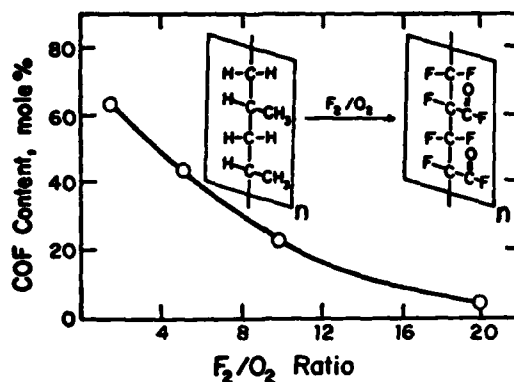
The relationship between oxygen introduced and the COF content (polypropylene)
