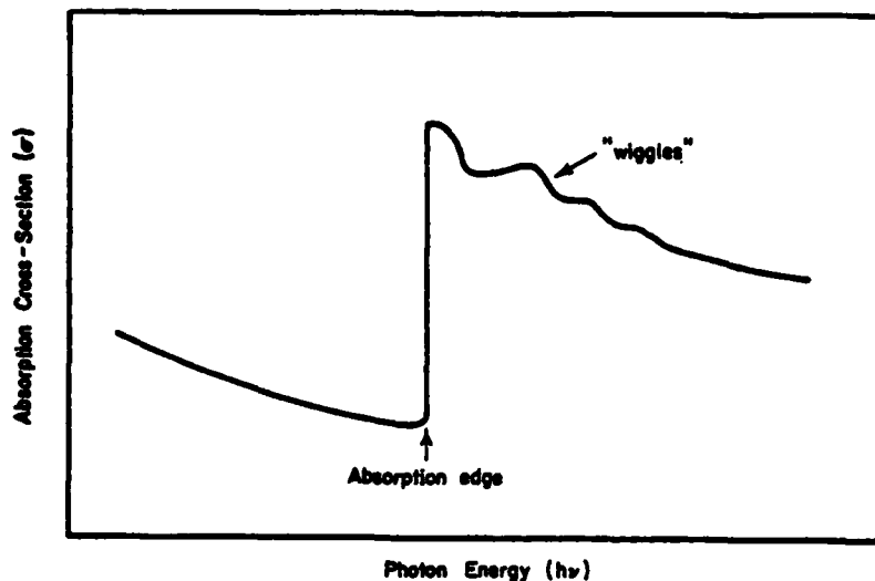
FIGURE 1. SCHEMATIC ILLUSTRATION OF AN EXTENDED X-RAY ABSORPTION FINE STRUCTURE (EXAFS) SPECTRUM
