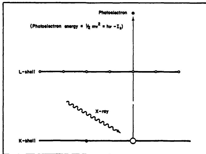
FIGURE 2. SCHEMATIC ILLUSTRATION OF ELECTRON SPECTROSCOPY FOR CHEMICAL ANALYSIS (ESCA).
