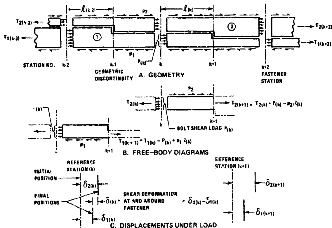
FIGURE 24. LOADS AND DEFORMATIONS ON ELEMENTS OF BOLTED JOINT
