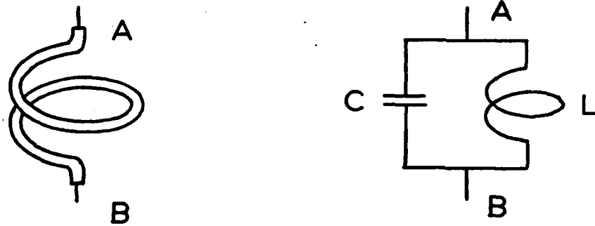
Fig. 2. (a) Cablechoke (b) Equivalent circuit
