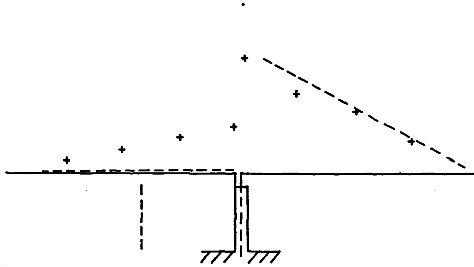
Fig. 1. Horizontal dipole with unbalanced currents; --- computed + measured
