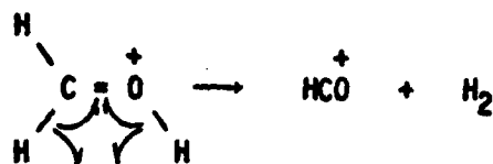
SCHEME 13: [31]^+ \rightarrow [29]^+
