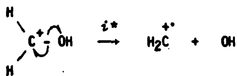
SCHEME 14: [31]^+ \rightarrow [14]^+
