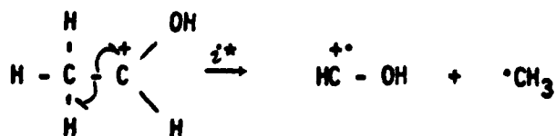
SCHEME 4: [45]^{\cdot+} \rightarrow [30]^{\cdot+}
