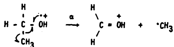
SCHEME 2: [46]^{\cdot+} \rightarrow [31]^+
