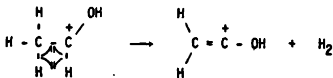
SCHEME 3: [45]^{\cdot+} \rightarrow [43]^+
