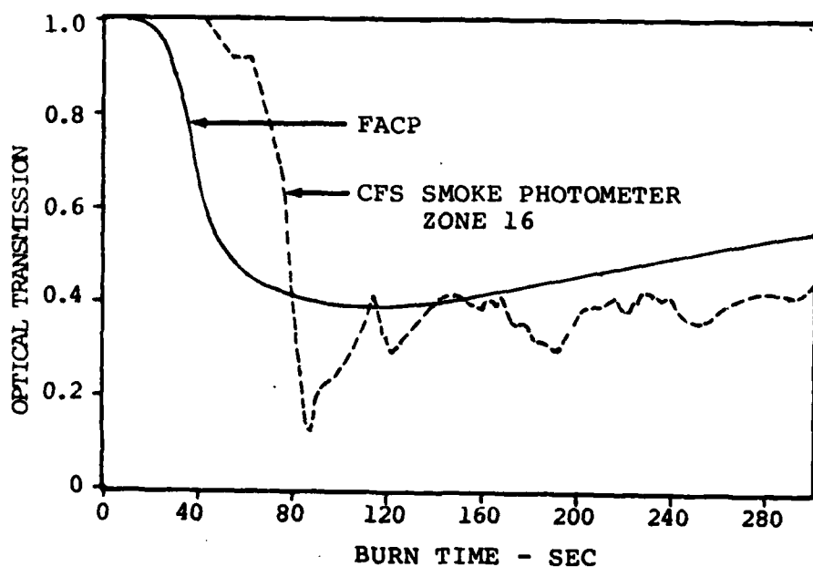
FIGURE 52. COMPARISON OF SMOKE EVOLUTION PROFILES - SINGLE ZONE FACP PREDICTION WITH CFS EXHAUST READINGS FOR PANEL 2 AT 2.2 \text{ Btu/ft}^2 \text{ SEC}
