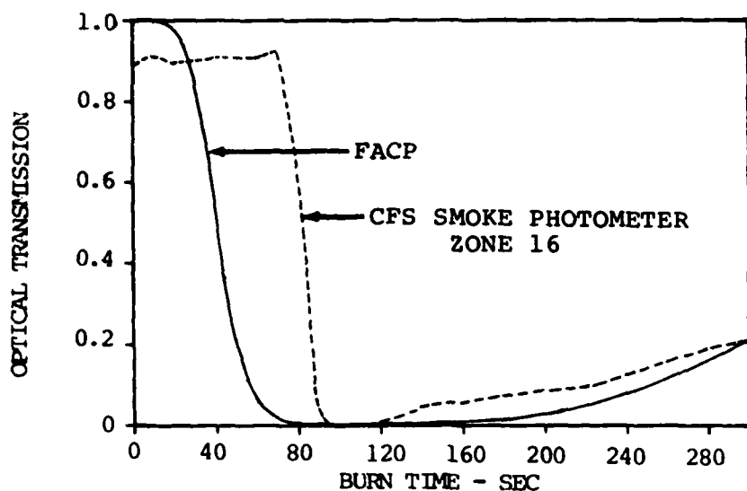
FIGURE 51. COMPARISON OF SMOKE EVOLUTION PROFILES - SINGLE ZONE FACP PREDICTION WITH CFS EXHAUST READINGS FOR PANEL 4 AT 2.2 \text{ Btu/ft}^2 \text{ SEC}
