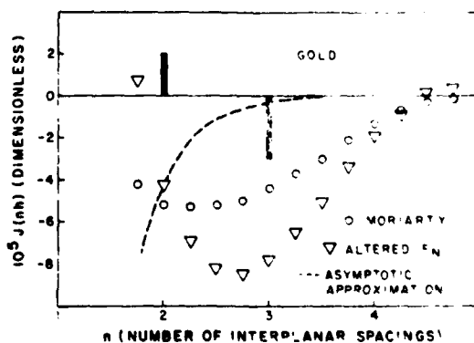
FIG. 6. Interplanar potential functions for gold. The corresponding energy-wave-number characteristics are shown in Fig. 2.
