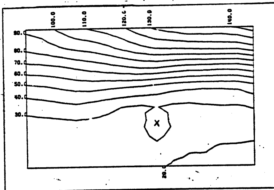
Fig. 2-2. The mean (composite) D-value field at 500mb. Isopleths are deviation in meters from standard atmosphere. Storm is always located at grid point 70 (X).
