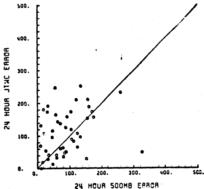
Fig. 5-1. Comparison of the forecast error for the independent data cases. Schemes compared are the 500mb EOF regression scheme versus the JTWC official forecast, for a 24 hour forecast. Units are in nautical miles.
