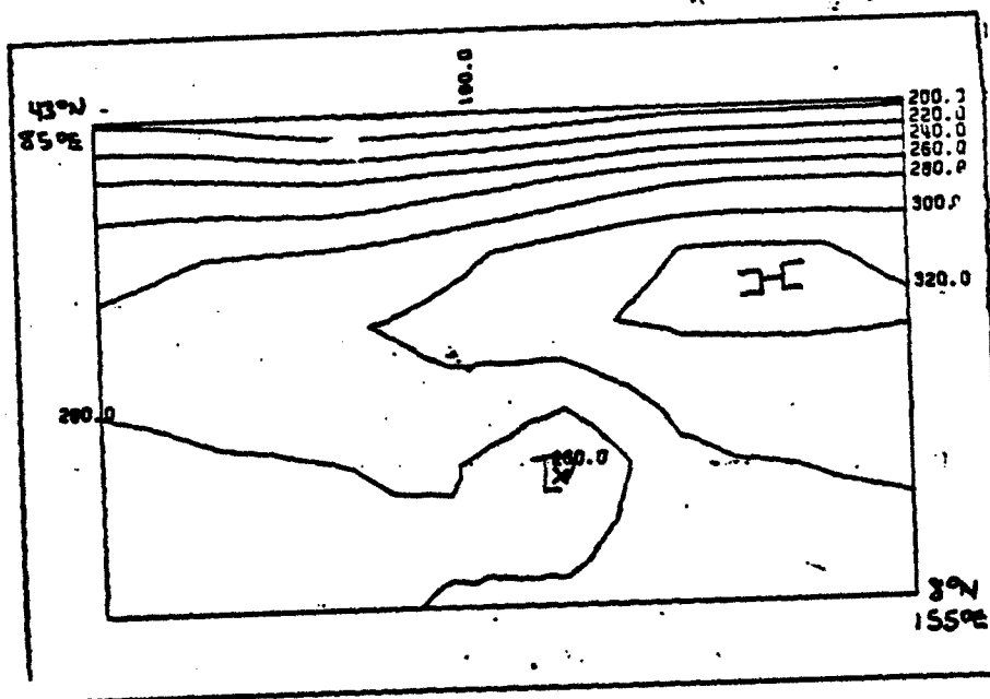
Fig. 4-13. Reconstruction of 500mb D-value field, 0000GMT 27 August 1967, using the first eigenvector and orthogonal coefficient. This compares to true field (Fig. 4-12).
