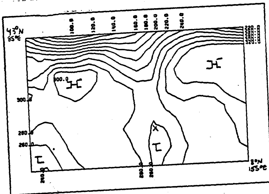
Fig. 4-12. 500mb D-value (meters) field surrounding Typhoon Marge at 0000GMT 27 August 1967. Marge is located at 18°N 125°E (location X).
