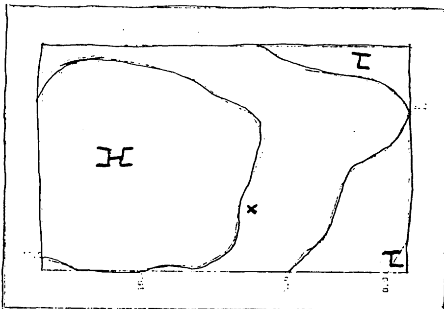
Fig. A1-11. Similar to Fig. A1-1 except for 850mb level.
