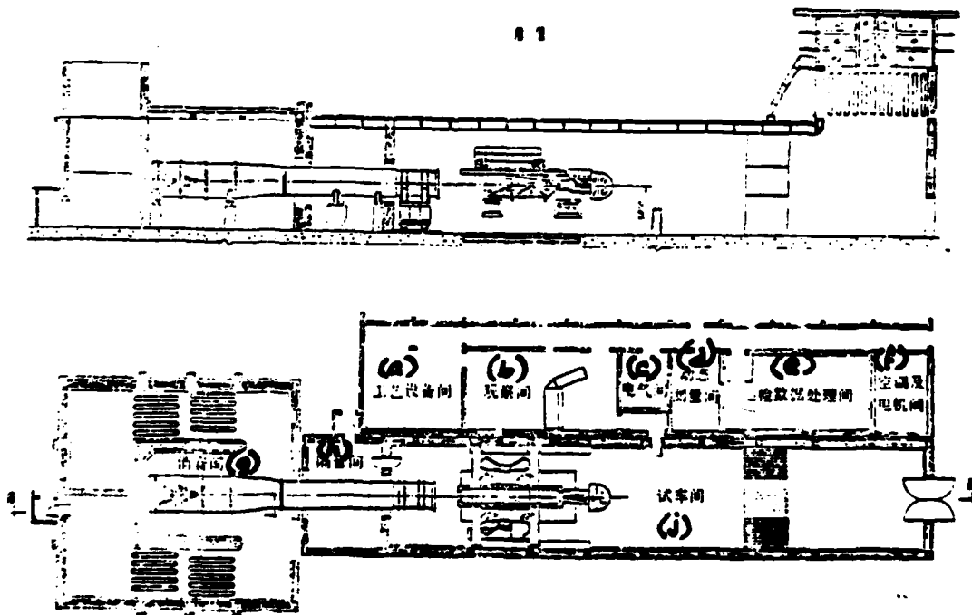
Fig. 1. Technical drawings of China's newly designed aircraft engine test stand
