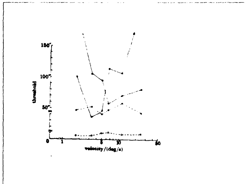
Figure 6. The effect of blur on spatial and temporal interpolation as a function of velocity for a separation between the stations \Delta x = 15' . Vernier resolution of a spatial offset is measured with (●) and without blur (○). Vernier resolution of a temporal offset is also shown with (○) and without (●) blur. The screen was blurred as described in the text. Notice that the first point for spatial offset is for v = 0' /sec. The observer is TV. The standard deviation is about 20% of the threshold values. From Fahle and Poggio (1981).
