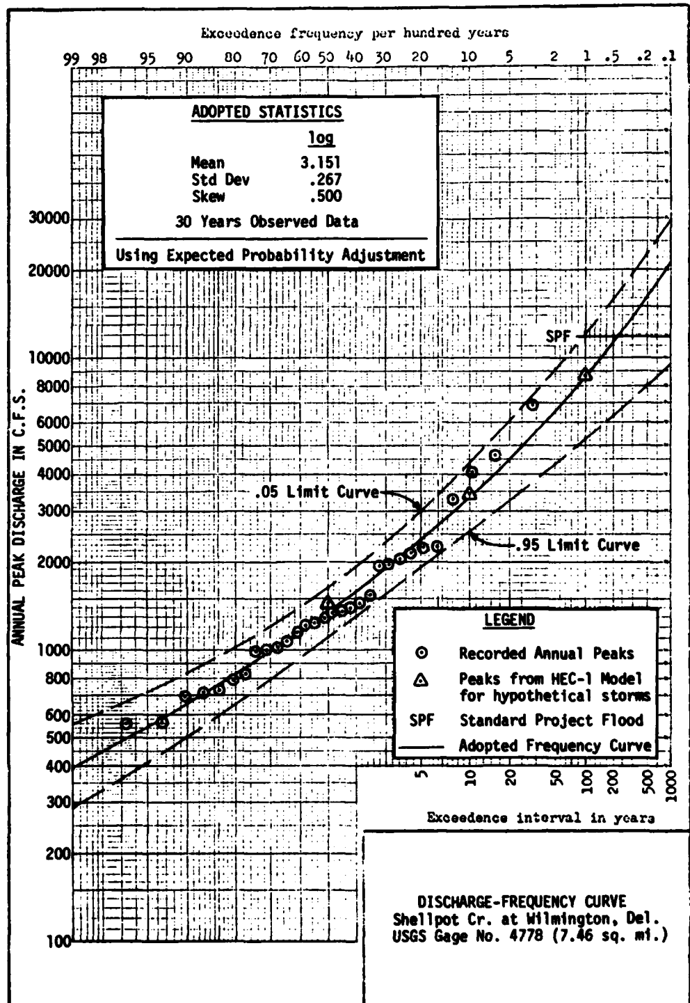
9.2. Discharge-Frequency Curve for Shellpot Creek
