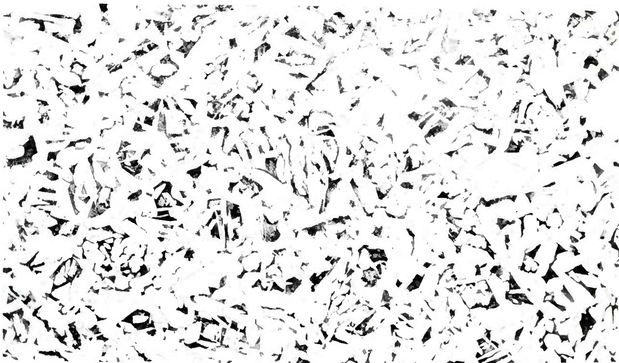
Figure 5. Microstructure at center of bar section 1A, picral etch - Republic Steel (100X)
