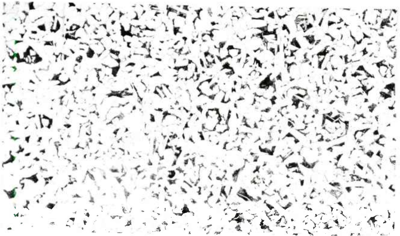
Figure 7. Microstructure at edge of bar section 1A, picral etch - Republic Steel (100X)
