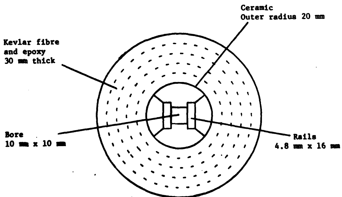
FIGURE 8. Cross-section of barrel: ERGS-2
