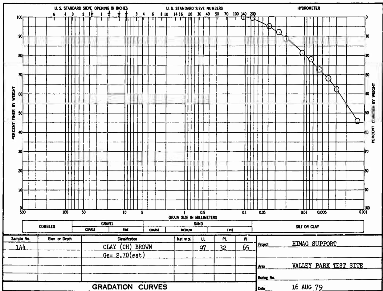
Figure C21. Gradation curve for site 7B, test series 139-144, sample 1A4
