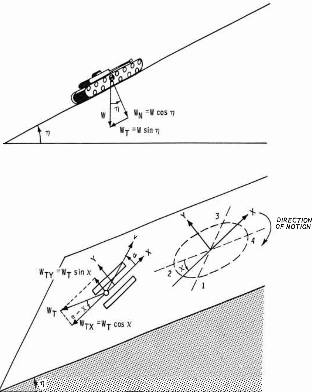
Figure A11. Effect of sloping terrain on transient motion
