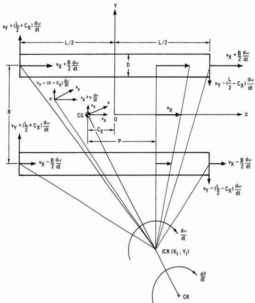
Figure A9. Track speeds and velocities of an arbitrary point of the hull
