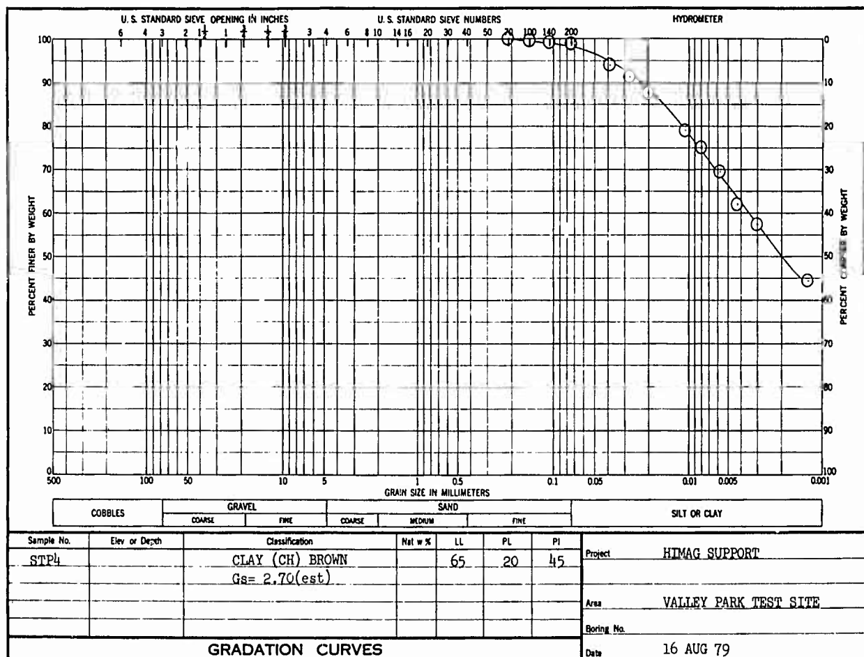
Figure C13. Gradation curve for site 7A, test series 131-134, sample STP4
