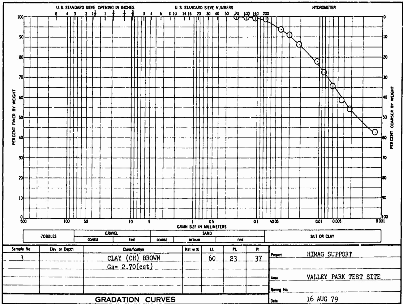
Figure C3. Gradation curve for site 7A, test series 98-102, sample 3
