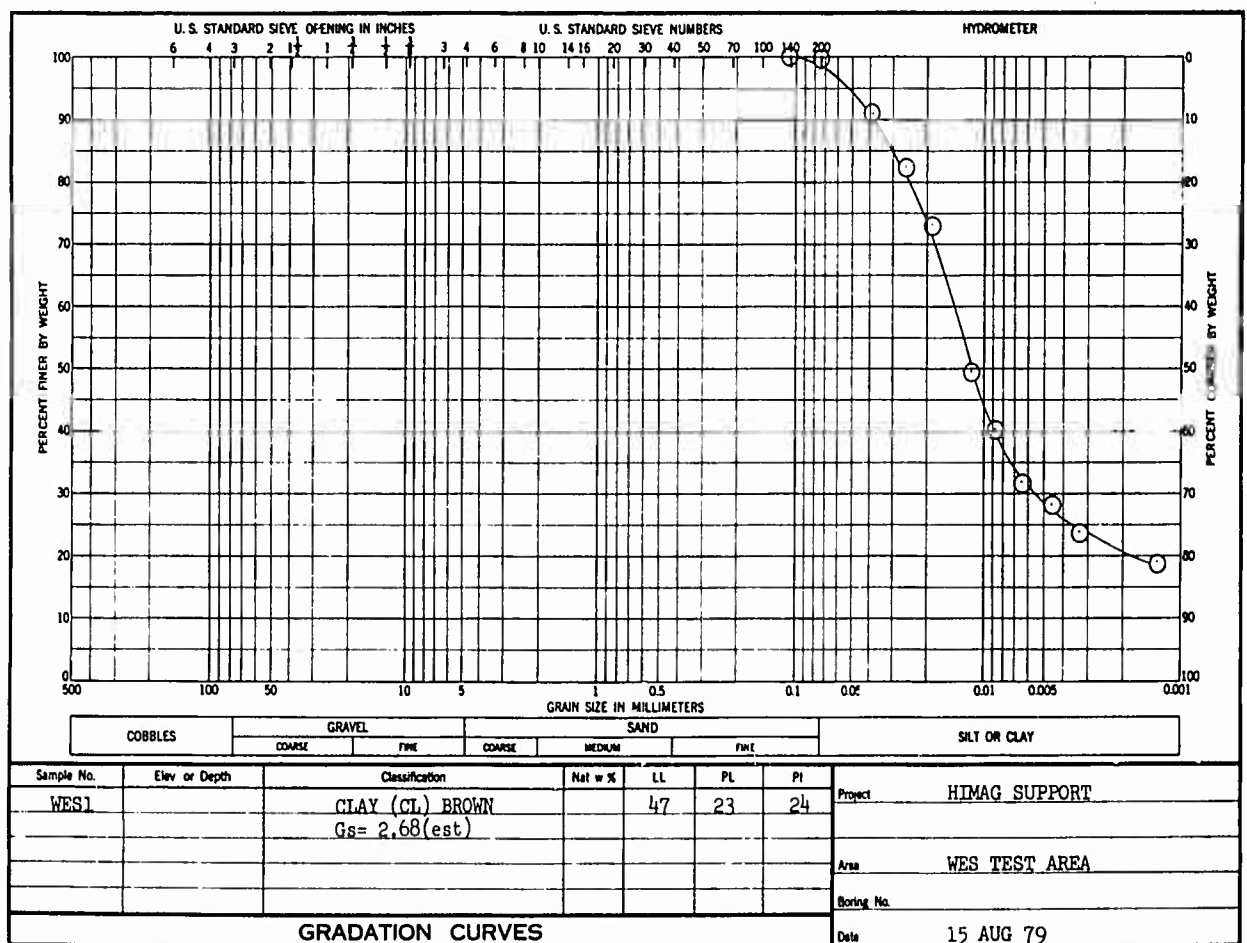
Figure C22. Gradation curve for site 8, test series 157-159, sample WES1
