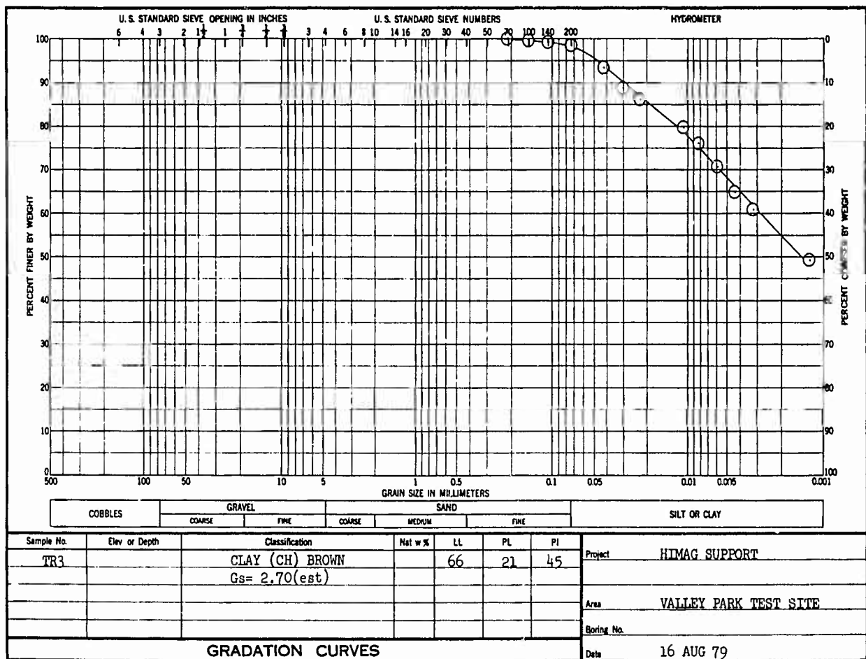
Figure C10. Gradation curve for site 7A, test series 131-134, sample TR3
