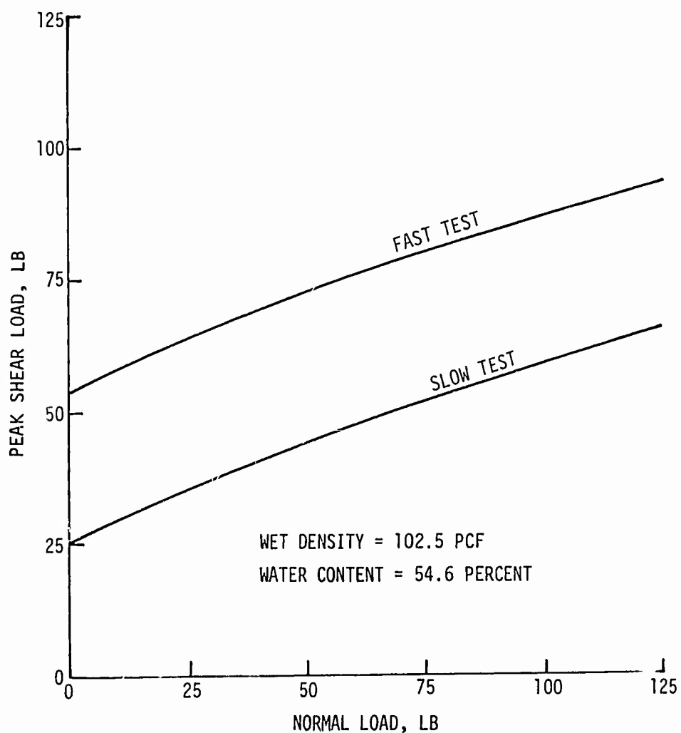
Figure 6. Peak shear load versus normal load (site 7B, test series 139-144)
