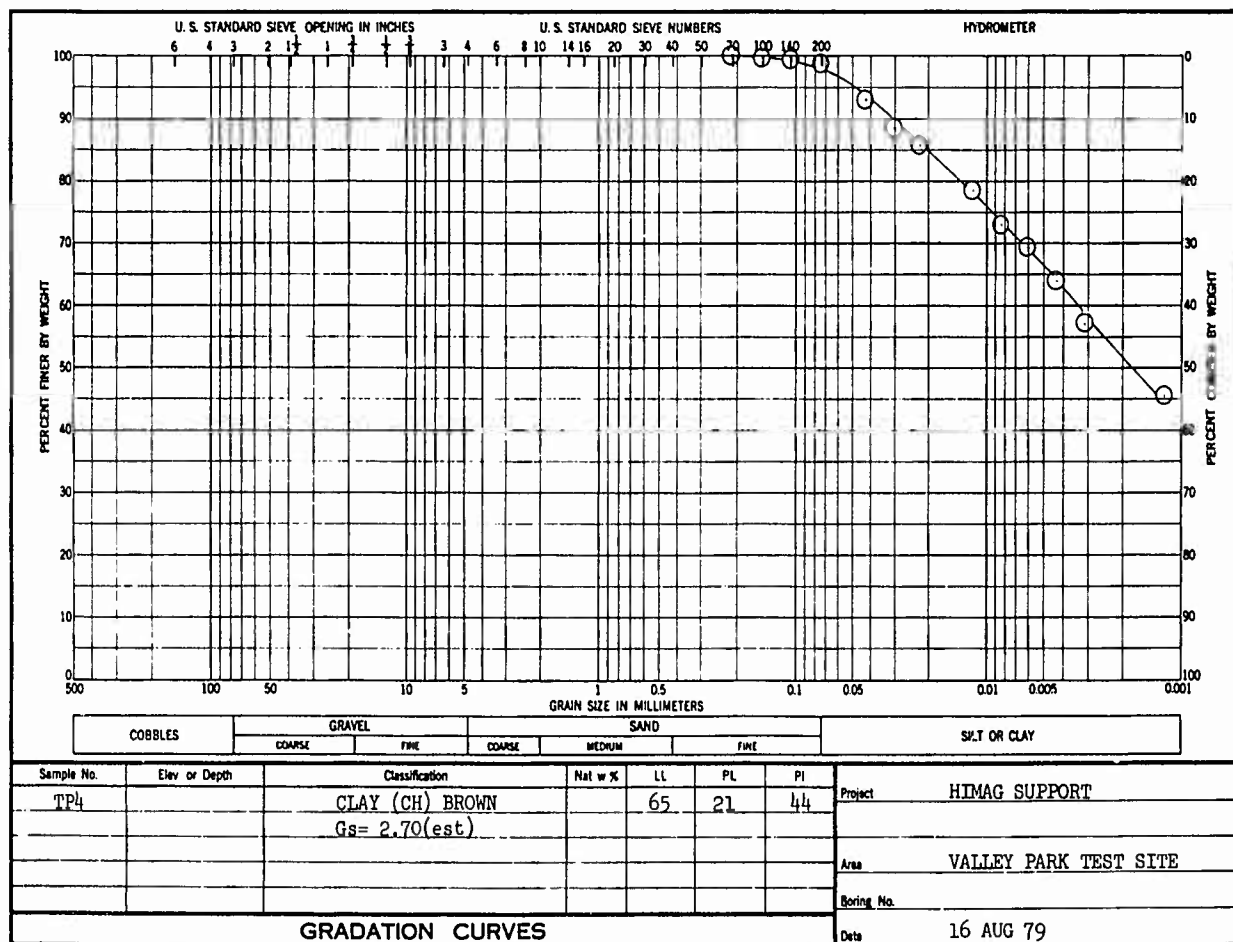
Figure C7. Gradation curve for site 7A, test series 117-122, sample TP4
