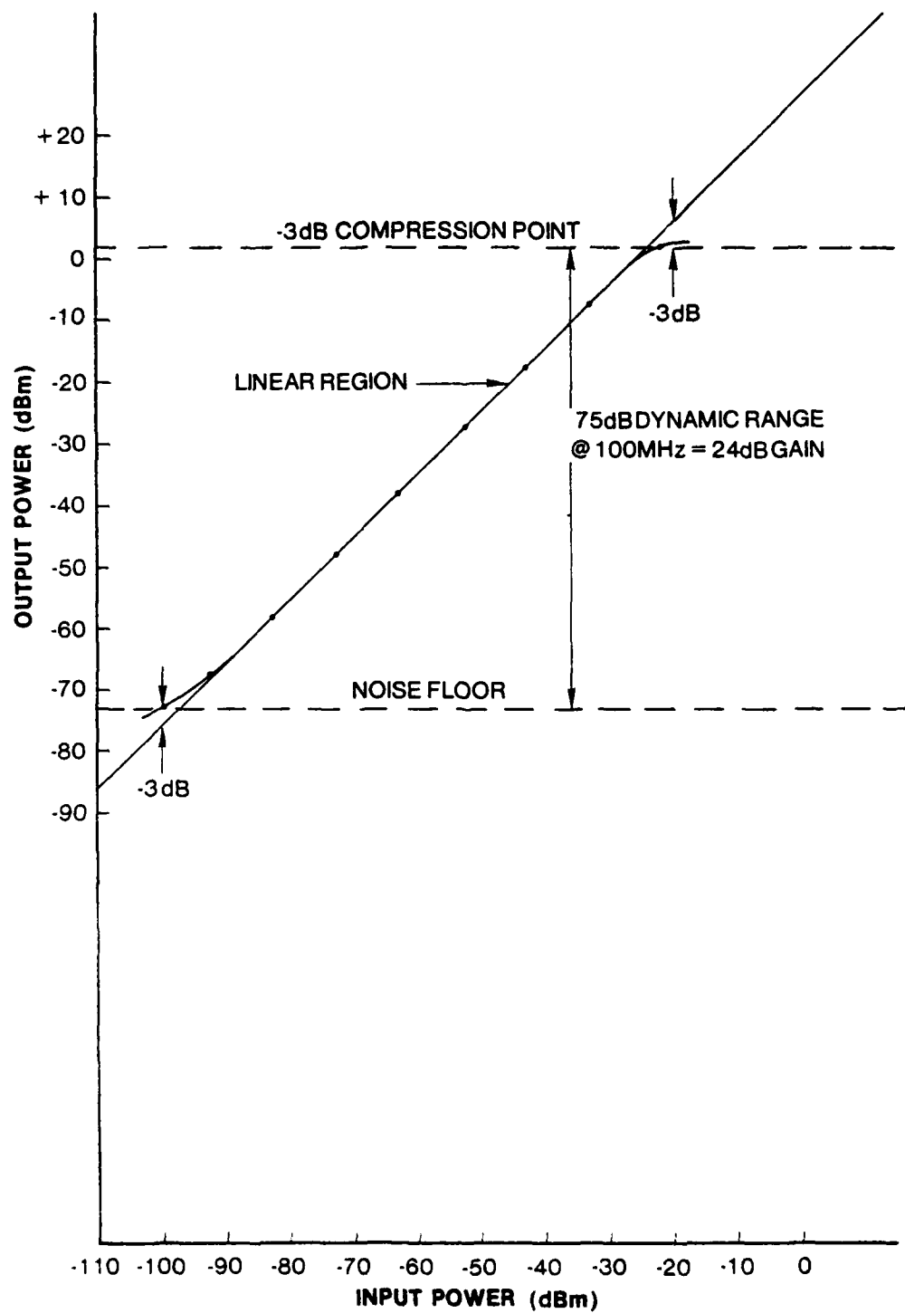
Figure 33. Variable Gain Amplifier Evaluation Plot of Output Power Versus Input Power at 100 MHz
