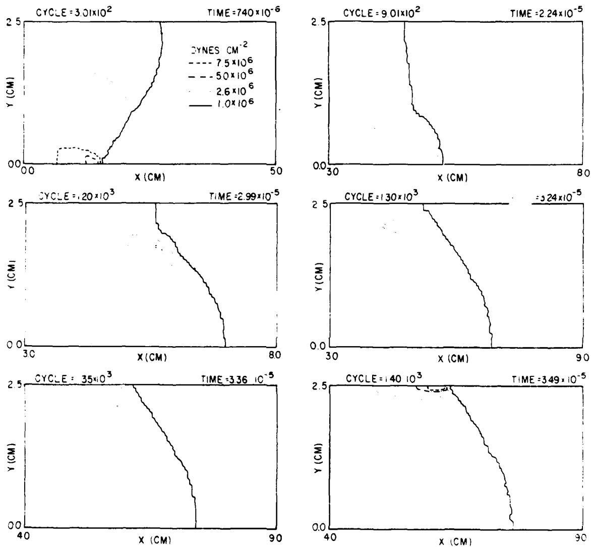
Fig. 3 — Pressure contours at selected times from a calculation of a detonation propagating in a stoichiometric H_2-O_2 mixture at 65 Torr and 298K in a tube 2.5 cm high. The legend is in the upper left hand box. The ragged edges of the surfaces are an artifact of the computer software.
