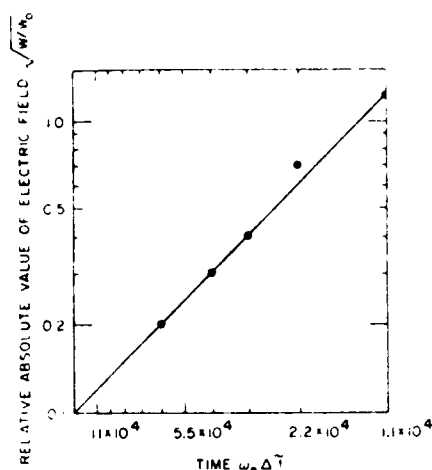
Fig. 16. Relative absolute value of electric field as a function of \omega_e \Delta t = \omega_e(t_0 + t) for the magnetized run. The collapse time, t_0 , is defined as the time at which the collapsing soliton would have reached singularity if there was no damping. \Delta t decreases toward the right so that real time is increasing toward the right. The value \omega_e t_0 corresponds to \omega_e t = 6.05 \times 10^5 in Figure 15.
