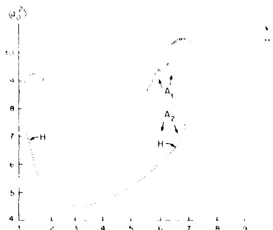
FIG. 4. Hysteresis: the long-time average of a_1 versus \gamma . [|||||]—chaotic behavior, ————limit cycles, ————stable stationary point. H indicates a Hopf bifurcation (A1 and A2 are labels used in the text).
