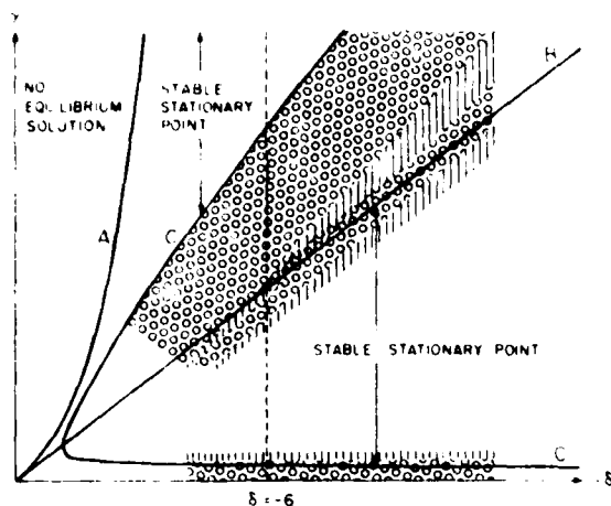
FIG. 2. Long-time asymptotic behavior of (5). [|||||]—chaotic behavior. [•••••]—limit cycles. Overlapping regions indicate the presence of two attractors. (The low \gamma region has been exaggerated for clarity. Curves A, B, and C are the same as in Fig. 1.)
