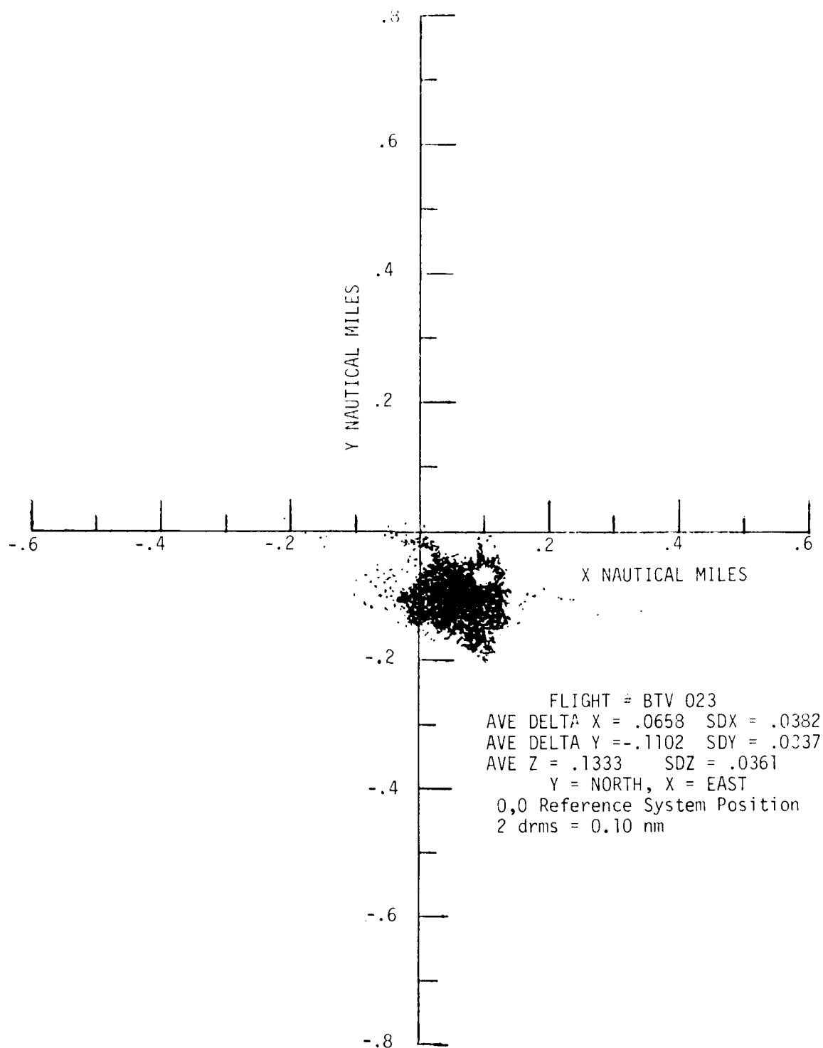
FIGURE 2.1-8. SCATTER PLOT FOR FLIGHT BTV 023
