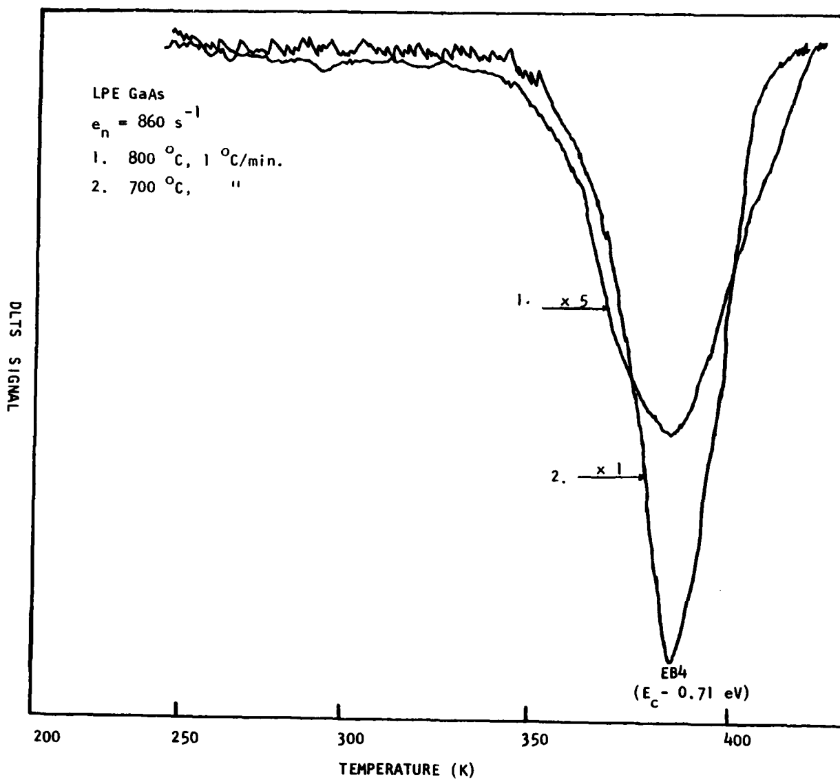
Fig. 7.13 DLTS scans of electron trap for two LPE GaAs samples grown at 700 and 800^\circ\text{C} with 1^\circ\text{C/min.} cooling rate.
