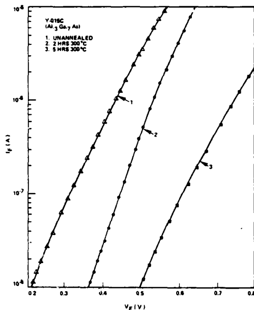
Fig. 3. The forward I-V characteristics curves for diodes Y-015C (Al 0.3 Ga 0.7 As), before and after 300 °C thermal annealing for 2 and 5 hrs..
