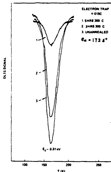
Fig. 7. DLTS thermal scans of the electron trap ( E_C - 0.31 \text{ eV} ) for three Y-015C diodes, unannealed and annealed at 300^\circ \text{C} for 2 and 5 hrs., respectively.
