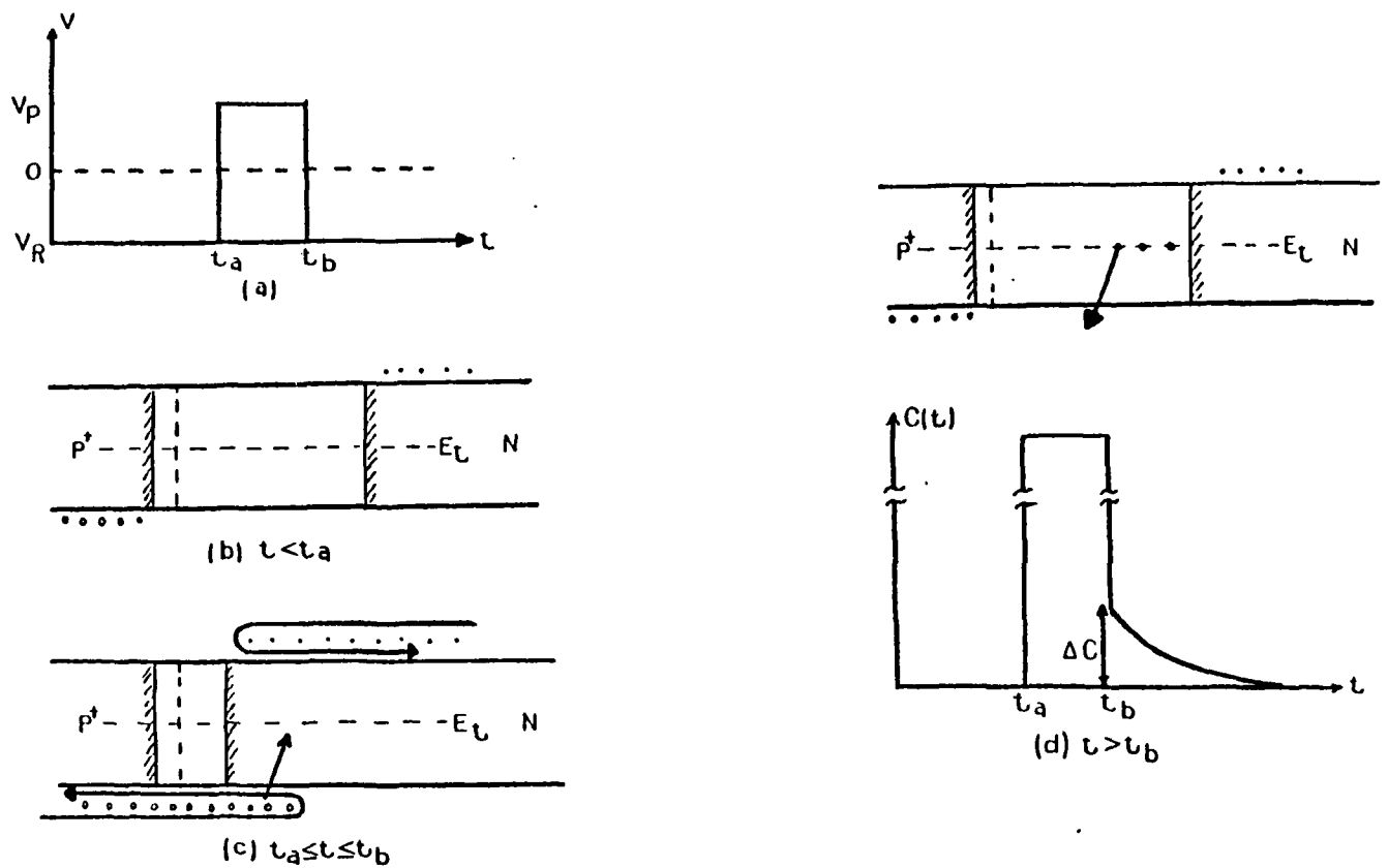
Fig. 7.1 Schematic diagrams of minority carrier injection process in a p-n diode in the DLTS measurement.
