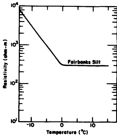
a. Resistivity of saturated Fairbanks silt vs temperature.
