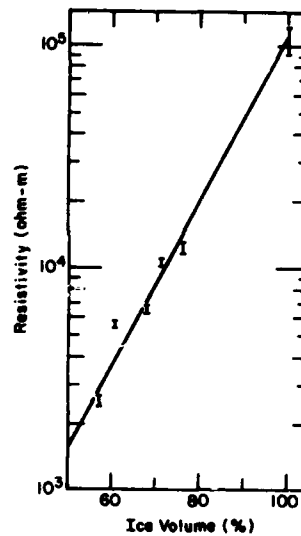
b. In-situ resistivity vs ice content of Fairbanks silt as measured in the wall of the CRREL Permafrost Tunnel.
