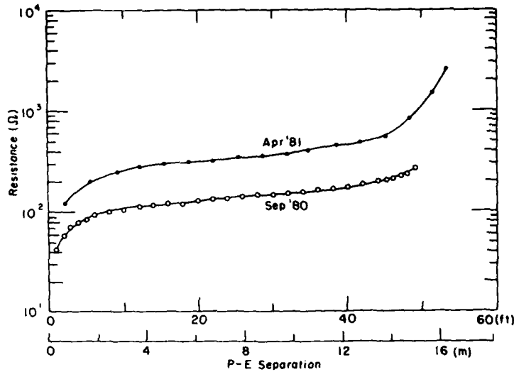
Figure 8. Resistance to ground of electrode 3 for two seasons.
