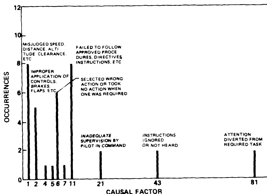
Figure 3-23. Crew Errors—Landing
