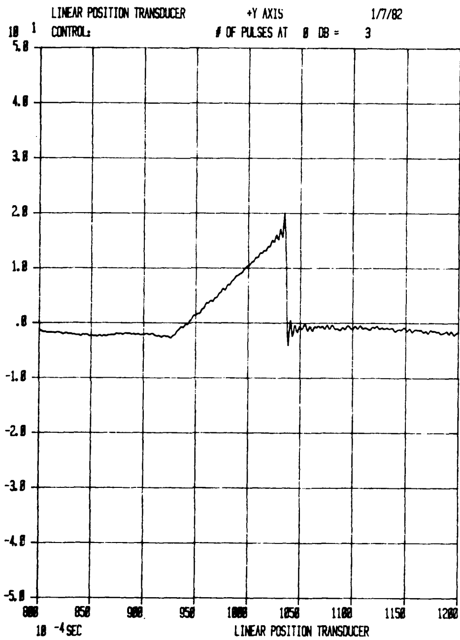
Figure E-4. Y-Axis MIL-STD-810C positive shock pulse.
