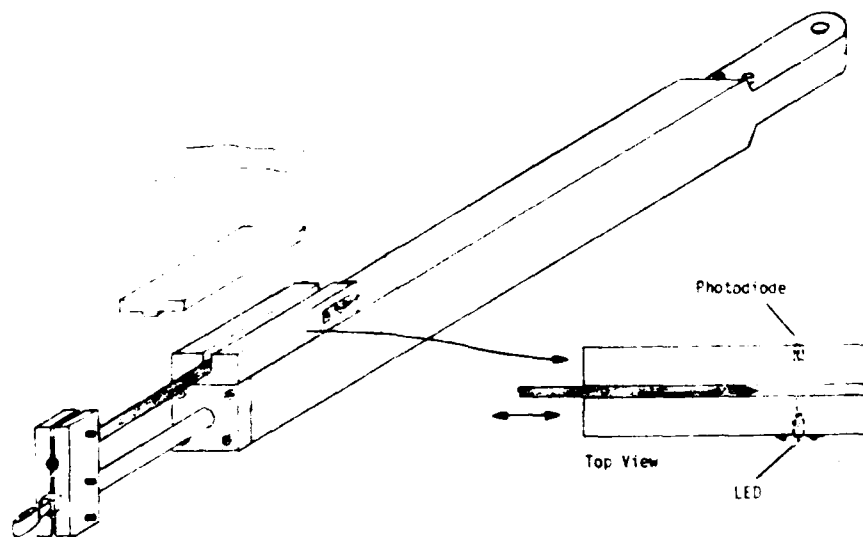
Figure 34. Dynamic accuracy test fixtures.
