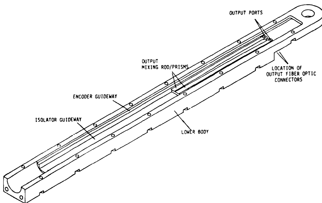
Figure F-3. Lower body details.
