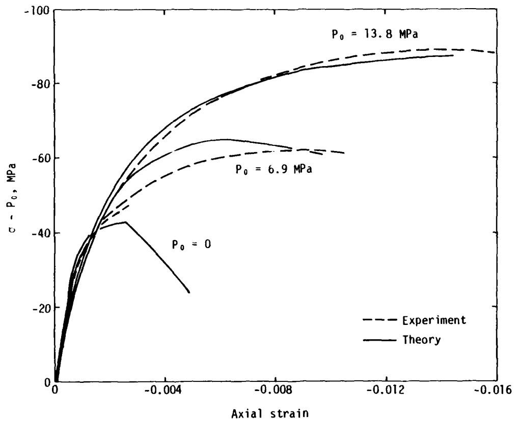
(a) Axial stress versus axial strain.
