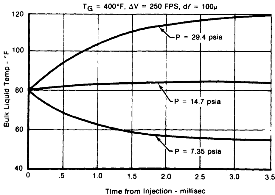
Figure 19. JP-4 Droplet Transient Temperature
