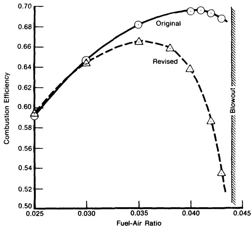
Figure 35. Revised Combustion Model Results, Fan Stream Case
