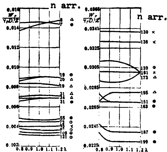
Fig. 13. \phi=0.98 \frac{W_p}{\gamma_p D_j^3 x} = \Omega(n, \text{arrangement}, \lambda) design curve
