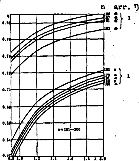
Fig. 9. \eta = \eta(n, \text{arrangement}, \lambda)
