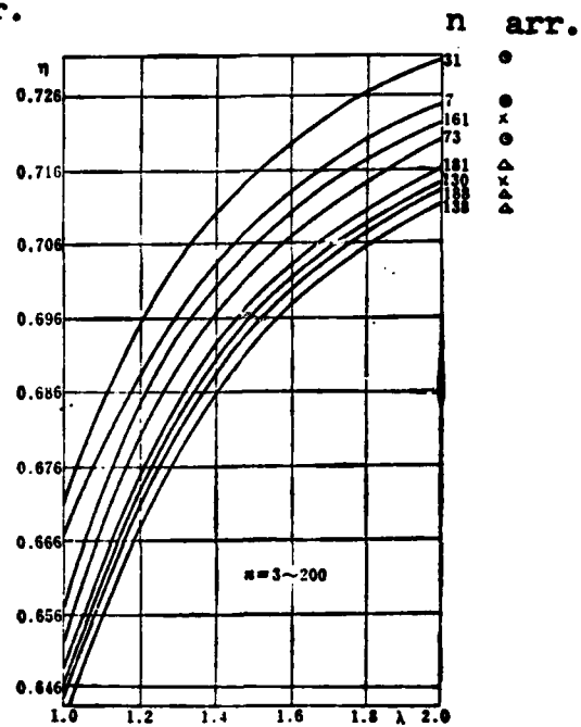
Fig. 4. \eta_I = \eta_I(n, \text{arrangement}, \lambda) Fig. 5. \eta_{II} = \eta_{II}(n, \text{arrangement}, \lambda)
