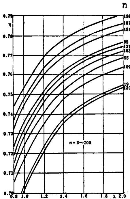
Fig. 4. \eta_I = \eta_I(n, \text{arrangement}, \lambda) Fig. 5. \eta_{II} = \eta_{II}(n, \text{arrangement}, \lambda)
