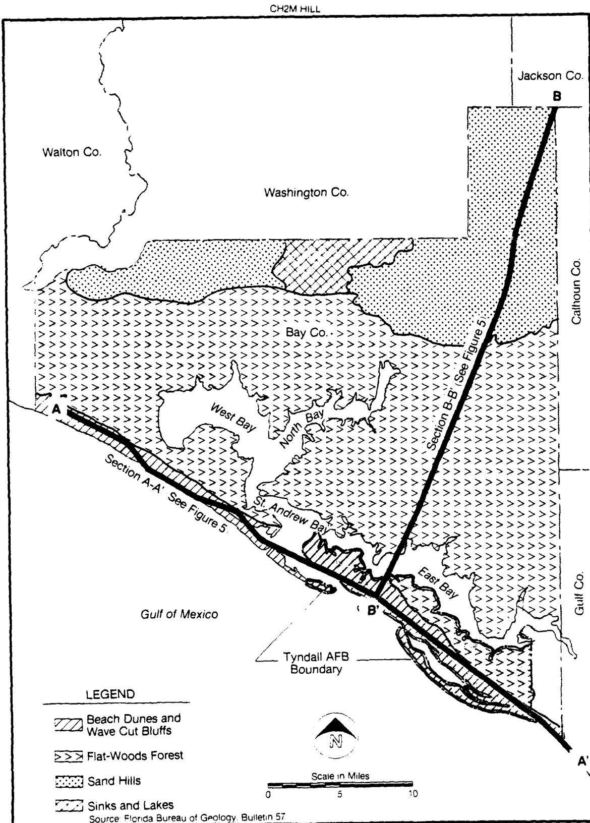
FIGURE 4. Physiographic subdivision map of Tyndall AFB.
