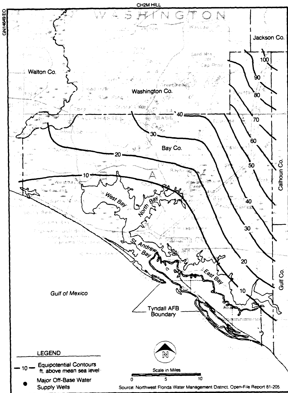
FIGURE 8. Potentiometric surface of the Floridan aquifer, 1980.
