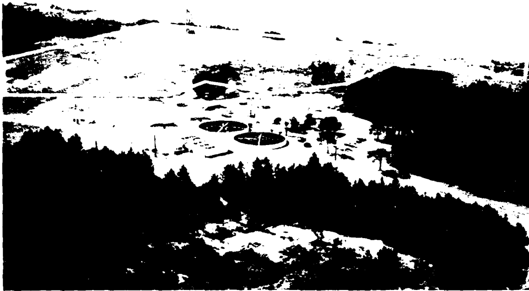
FIGURE K-1. Location of Tyndall AFB past landfill Site No. 6 (Sewage Plant Vicinity Landfill).
