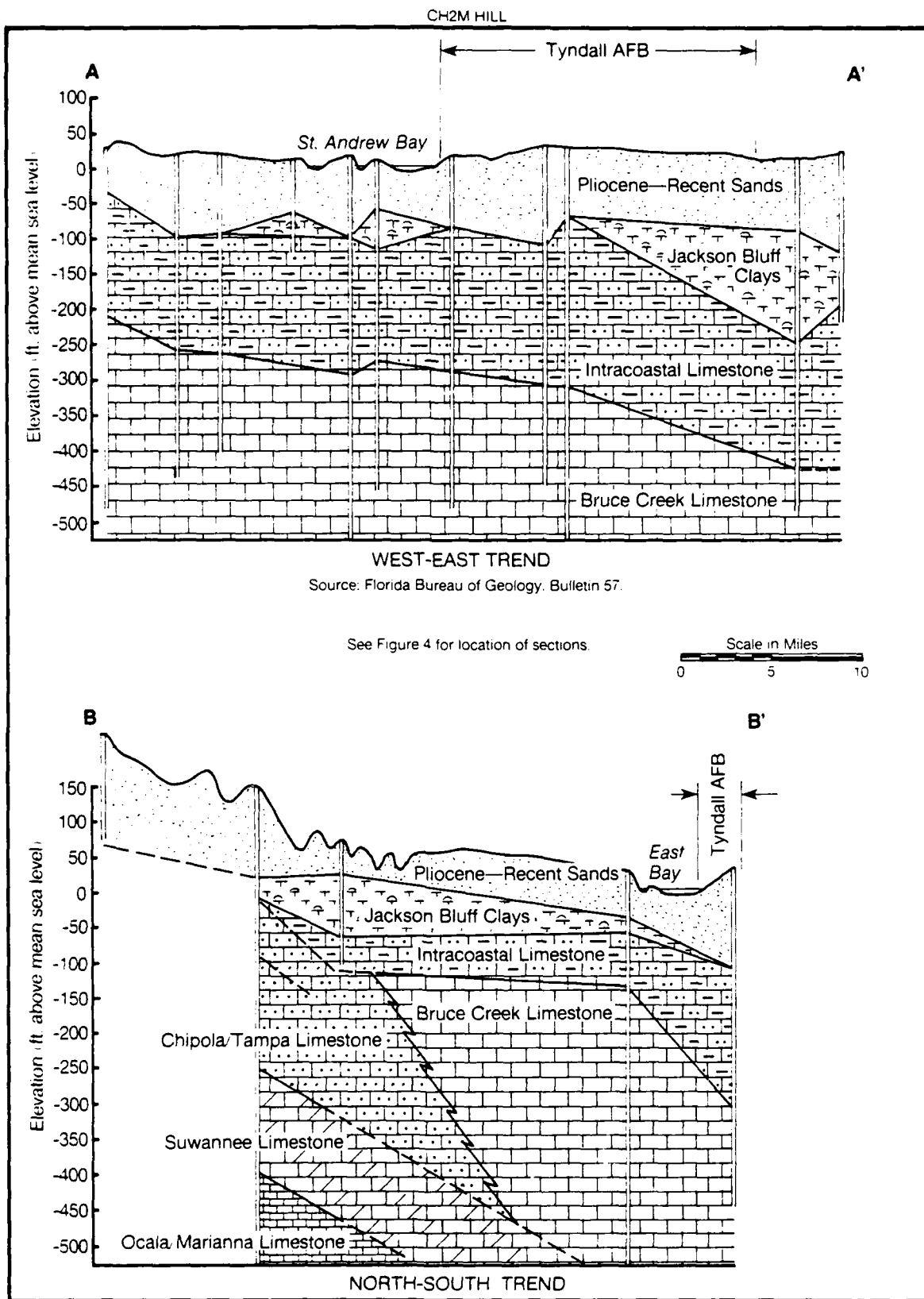
FIGURE 5. Typical geologic cross section of Tyndall AFB.
