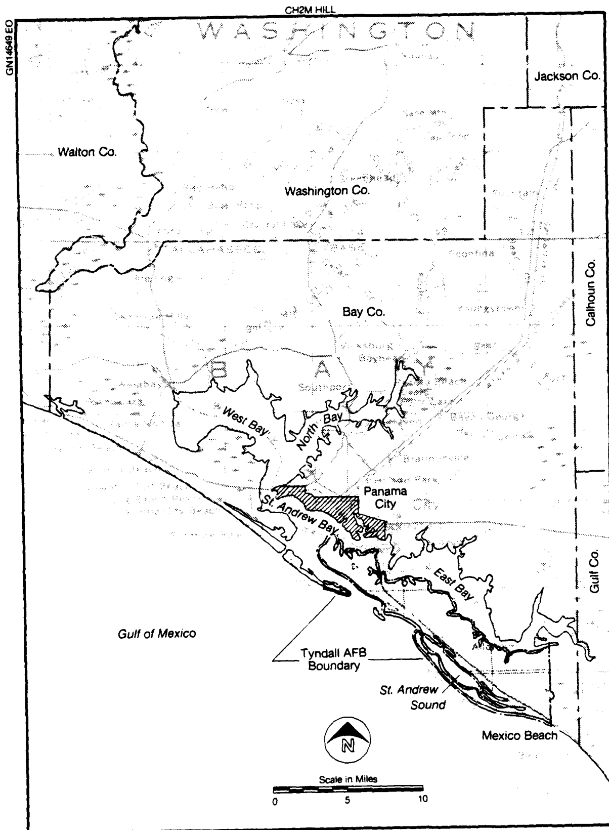
FIGURE 3. Location map of Tyndall AFB and contiguous surface-water bodies.
