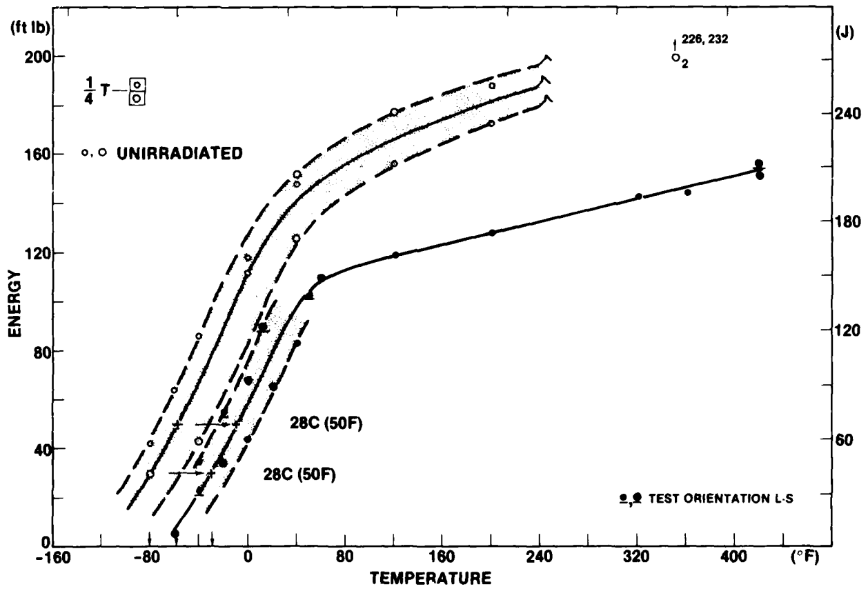
Fig. 8. Charpy-V notch ductility of the submerged arc weld, Code GW, supplied by the FRG.
