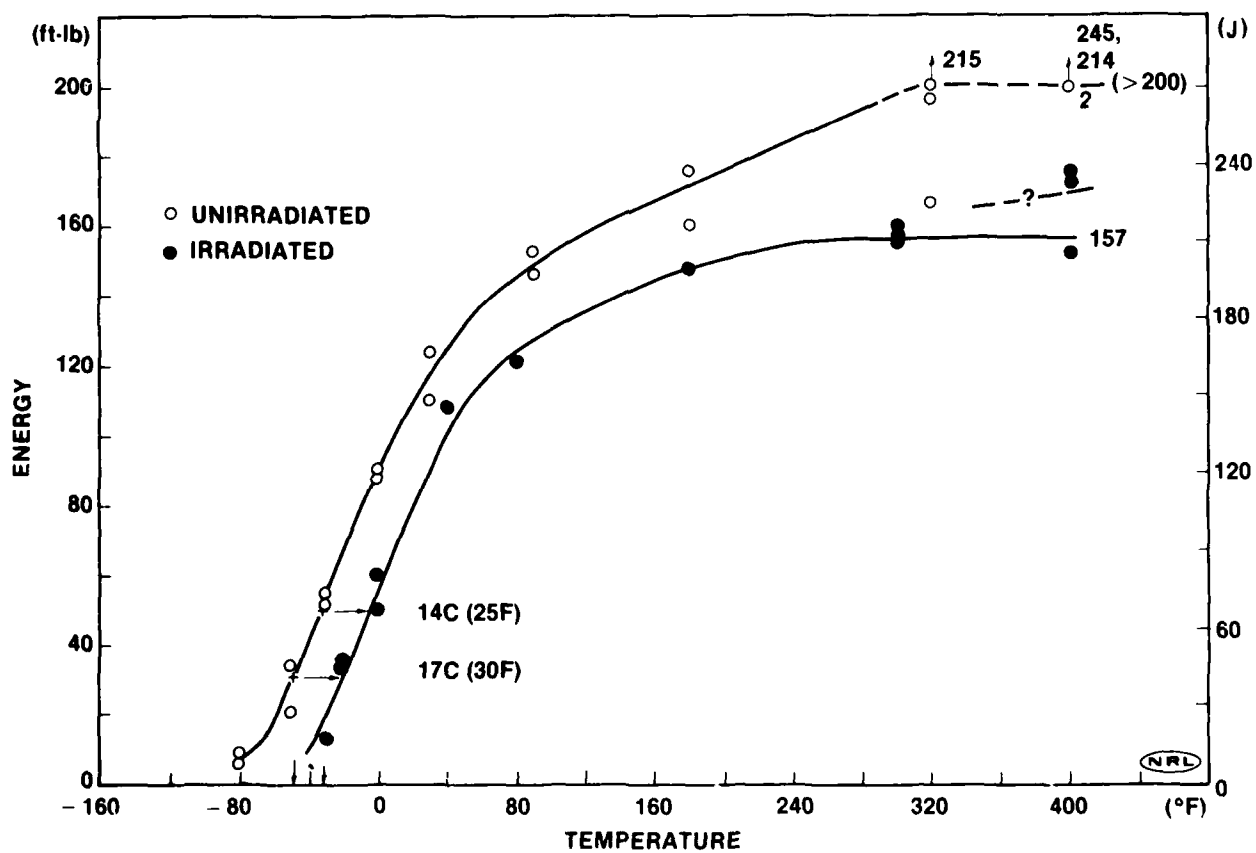
Fig. 1. Charpy-V notch ductility of the A533-B Class 1 steel plate, Code JP 107, supplied by Japan. In this Figure and in Figs. 2 through 9, the upper graph relates specimen lateral expansion and temperature while the lower graph relates specimen energy absorption and temperature.
