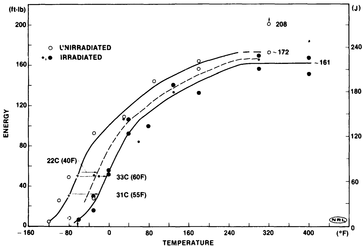
Fig. 2. Charpy-V notch ductility of the A508 Class 3 steel forging, Code JF 212, supplied by Japan.
