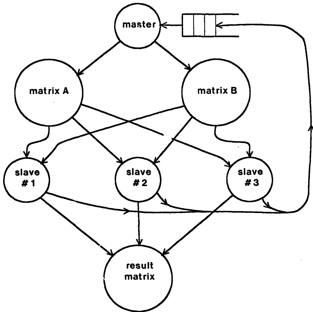
Figure 20: Structure of the MATR matrix multiplication program.
