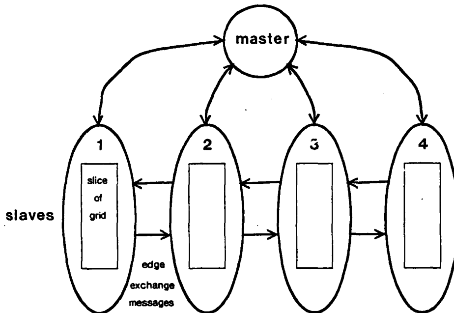
Figure 16: Structure of the PDES program.
