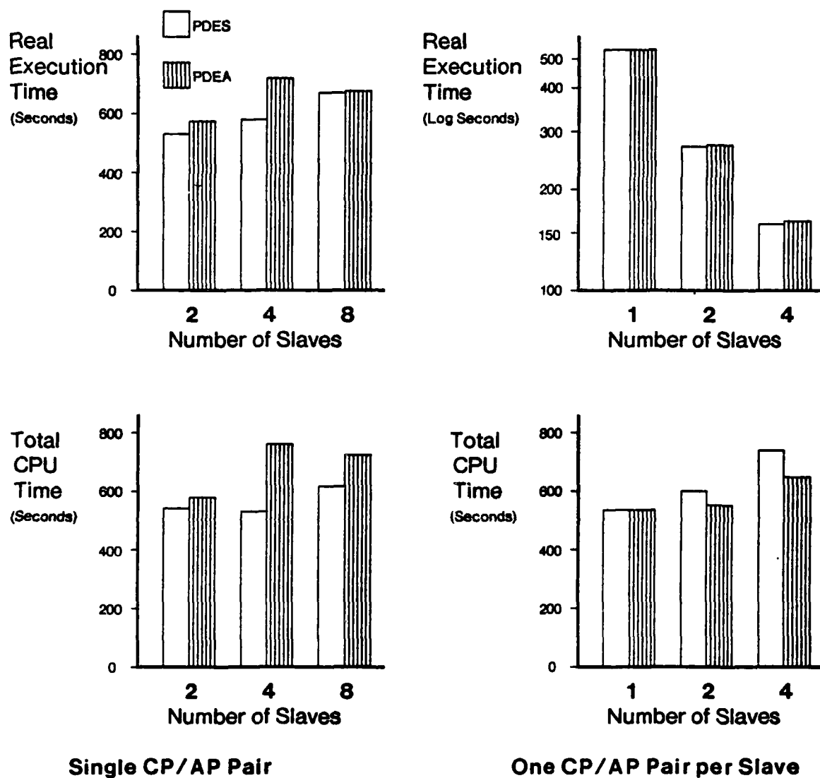
Figure 17: Measurements of the PDES and PDEA programs.
