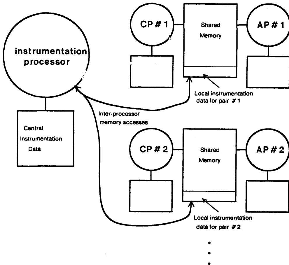
Figure 15: Instrumentation of the AMPL run-time system.
