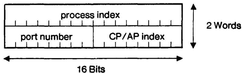
Figure 8: Representation of a process or port name.
