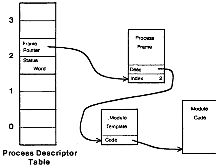
Figure 7: The process descriptor table.
