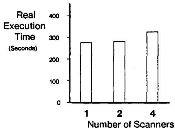
Figure 23: Execution times for the TELE program, using one CP/AP pair.
