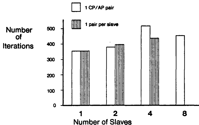
Figure 19: Number of iterations taken by the PDEA program.
