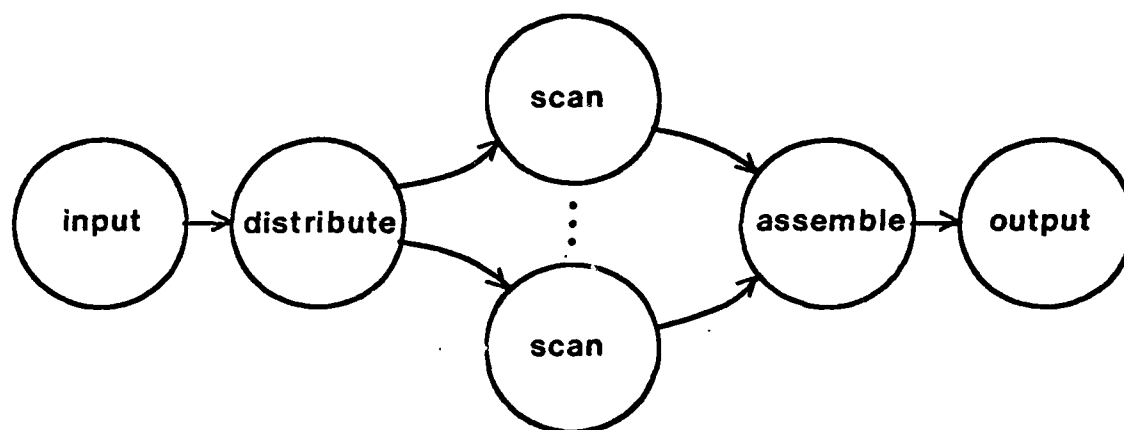
Figure 22: Structure of the TELE program.
