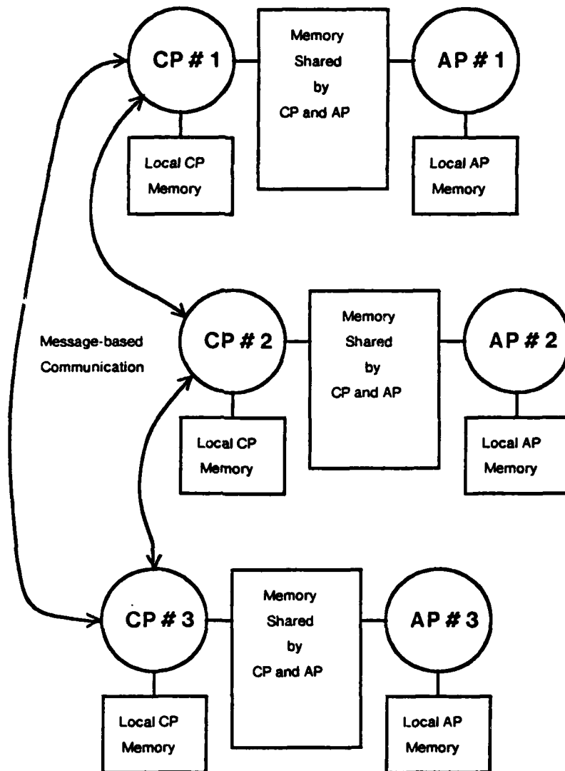
Figure 6: Basic structure of the run-time system.
