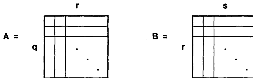
Figure 1: Two partitioned matrices.
