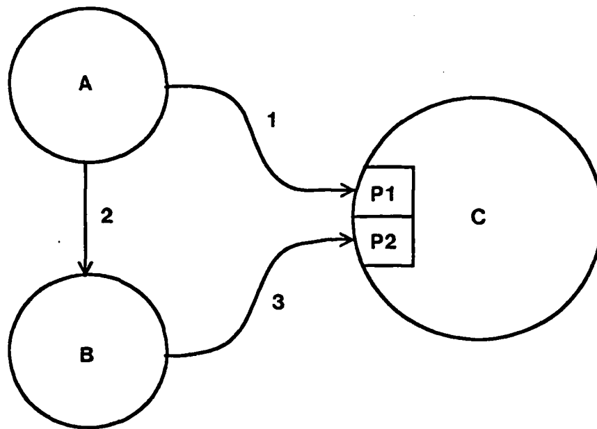
Figure 4: Synchronization of messages arriving at two ports.
