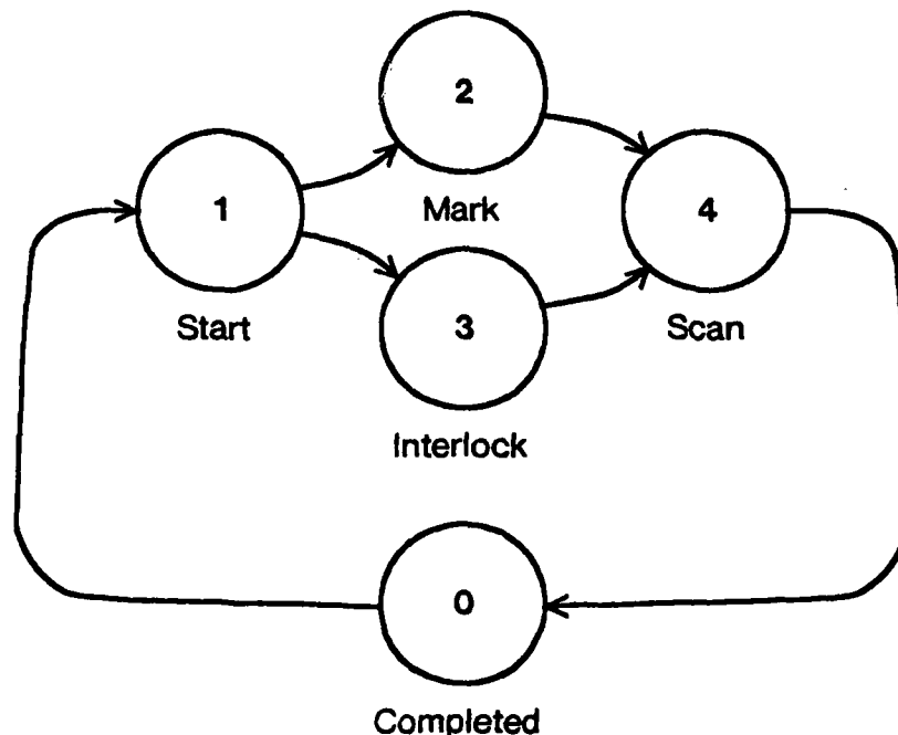
Figure 14: Garbage collection phases.
