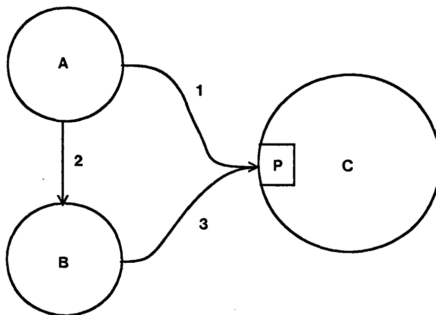
Figure 3: Two processes sending ordered messages to a single port.
