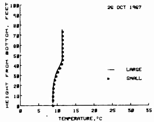
Plate 6X. Temperature profiles, pool el 1075.0, Jul-Oct 1967, with one additional level of large and small ports
