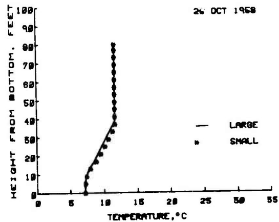
Plate 6J. Temperature profiles, pool el 1080.0, Jul-Oct 1958, with one additional level of large and small ports
