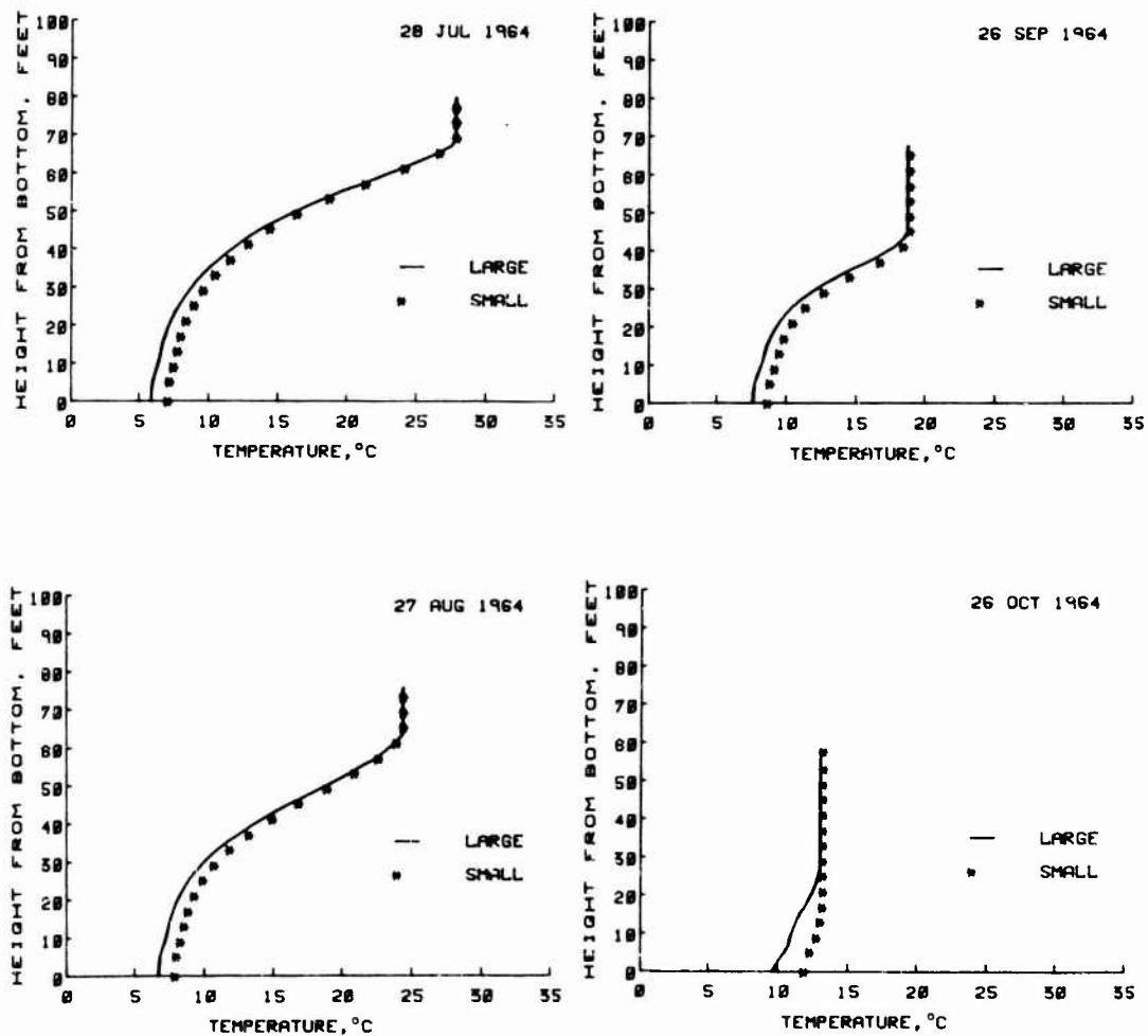
Plate 6L. Temperature profiles, pool el 1080.0, Jul-Oct 1964, with one additional level of large and small ports
