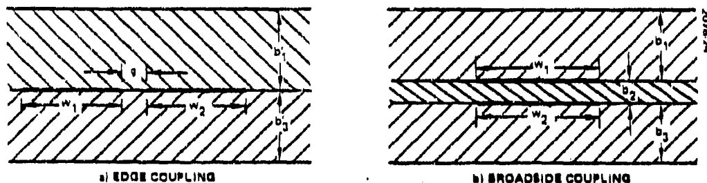
Figure 21. Stripline Configurations
