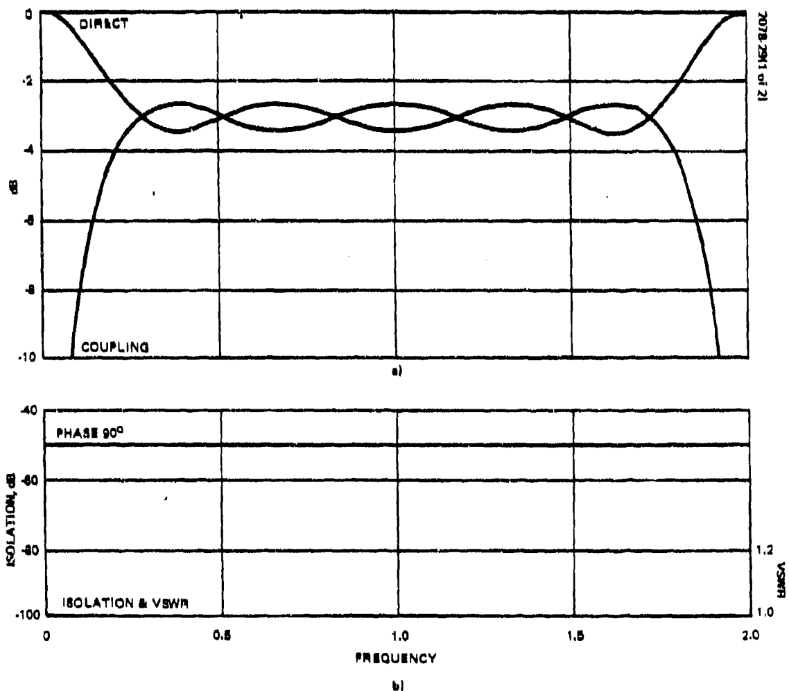
Figure 25. Response of Baseline Coupler
