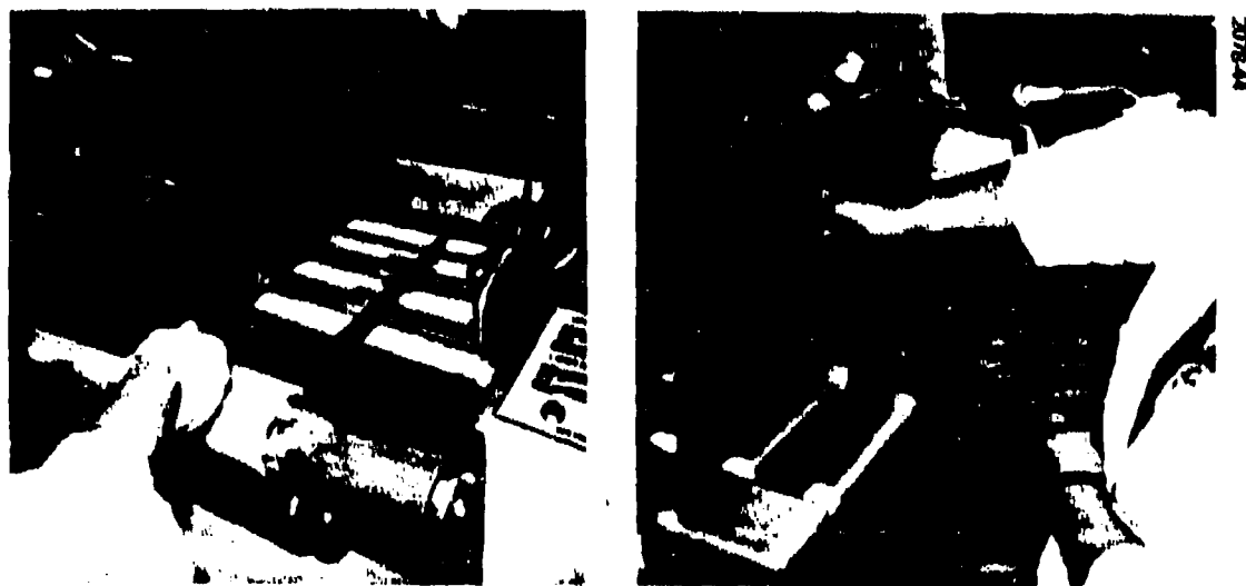
Figure 39. Resist Lamination Process
