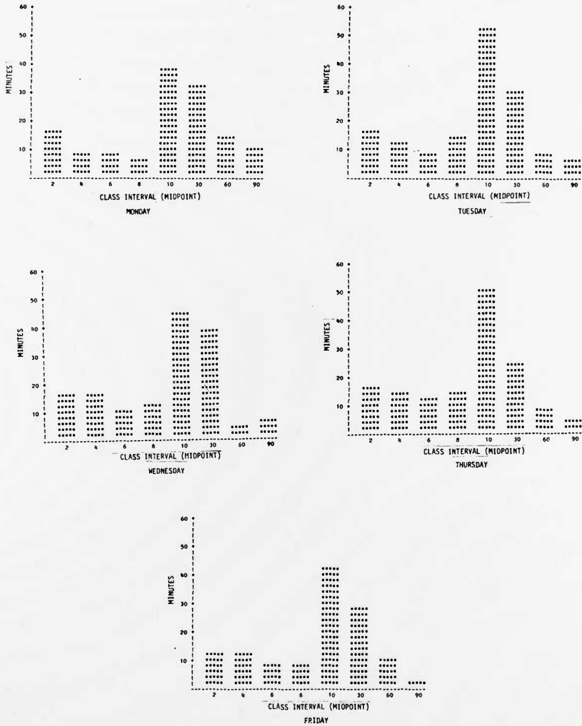
Figure A-5. Histogram of Mean Downtime by Day of Week
