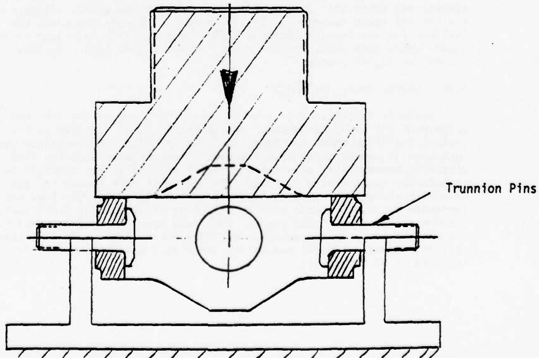
Figure 17 Ring Gimbal Trunnion Bore
