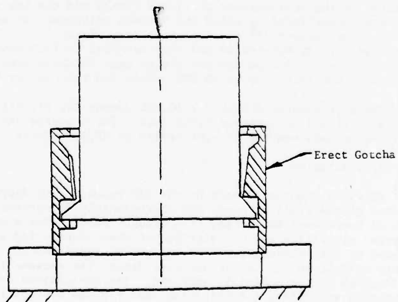
Figure 19 Gotcha Lock, Aft Teeth
