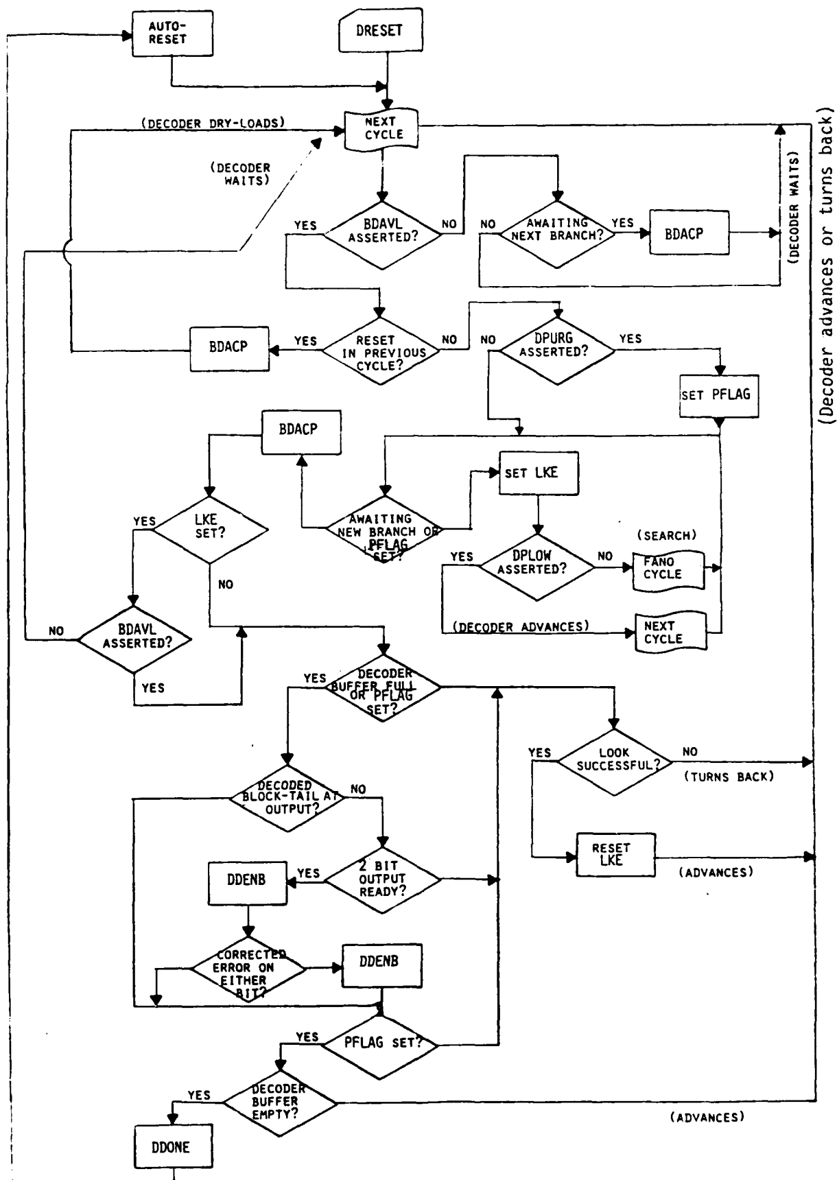
Figure 8-3. Contiguous Block Decoding Protocol
