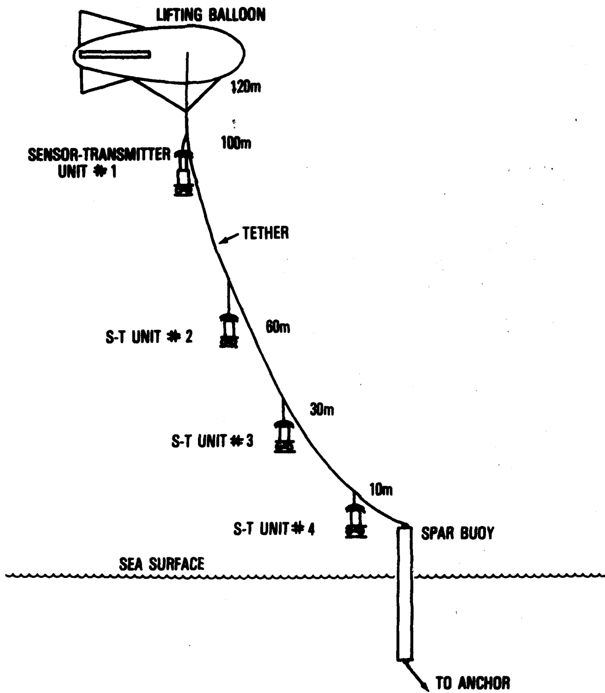
Figure 1.1 Sensor-Transmitter
