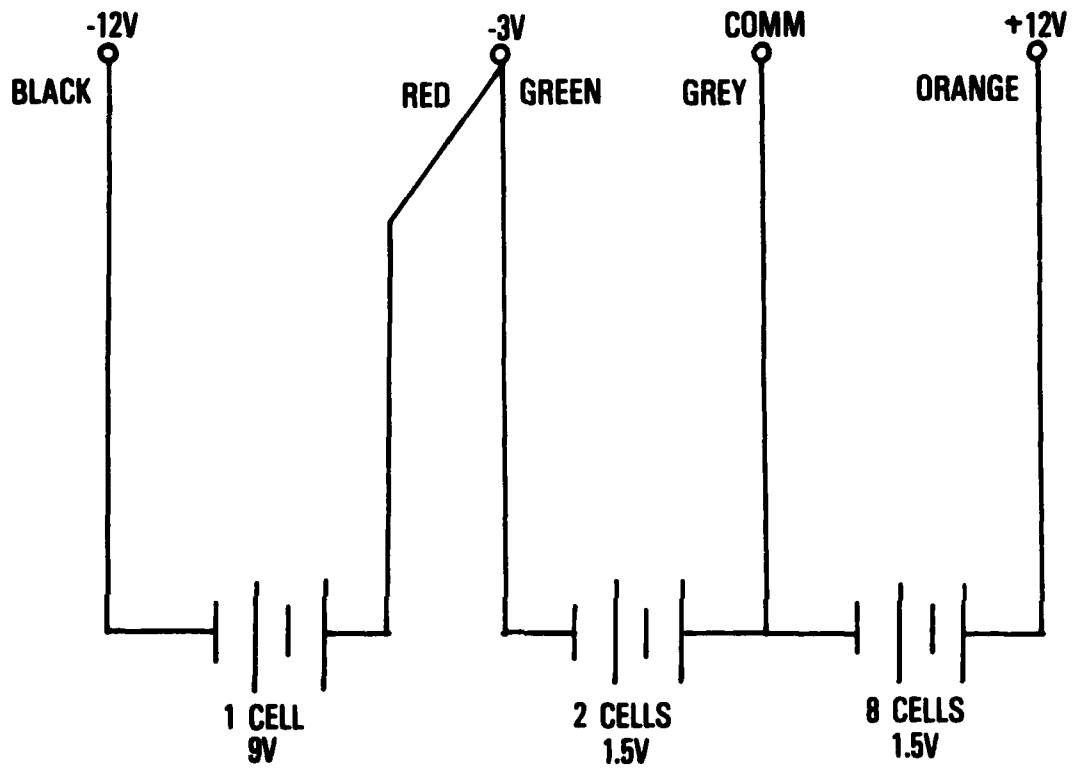
Figure 2.3 Battery Connections
