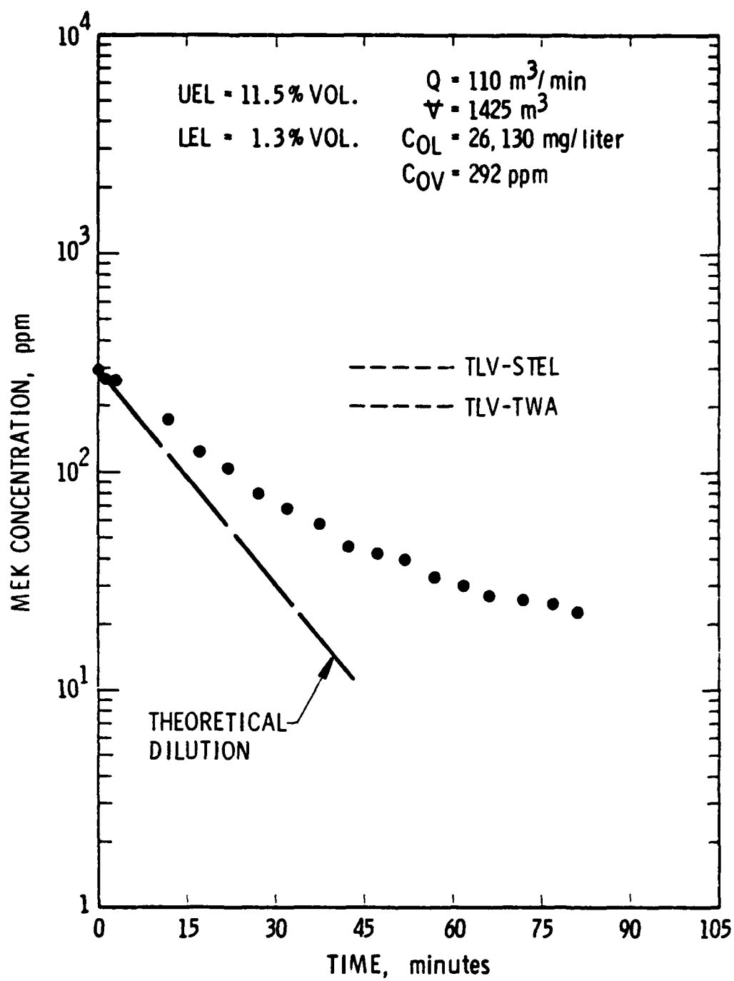
FIGURE 7. TANK VENTILATION OF 2CA
