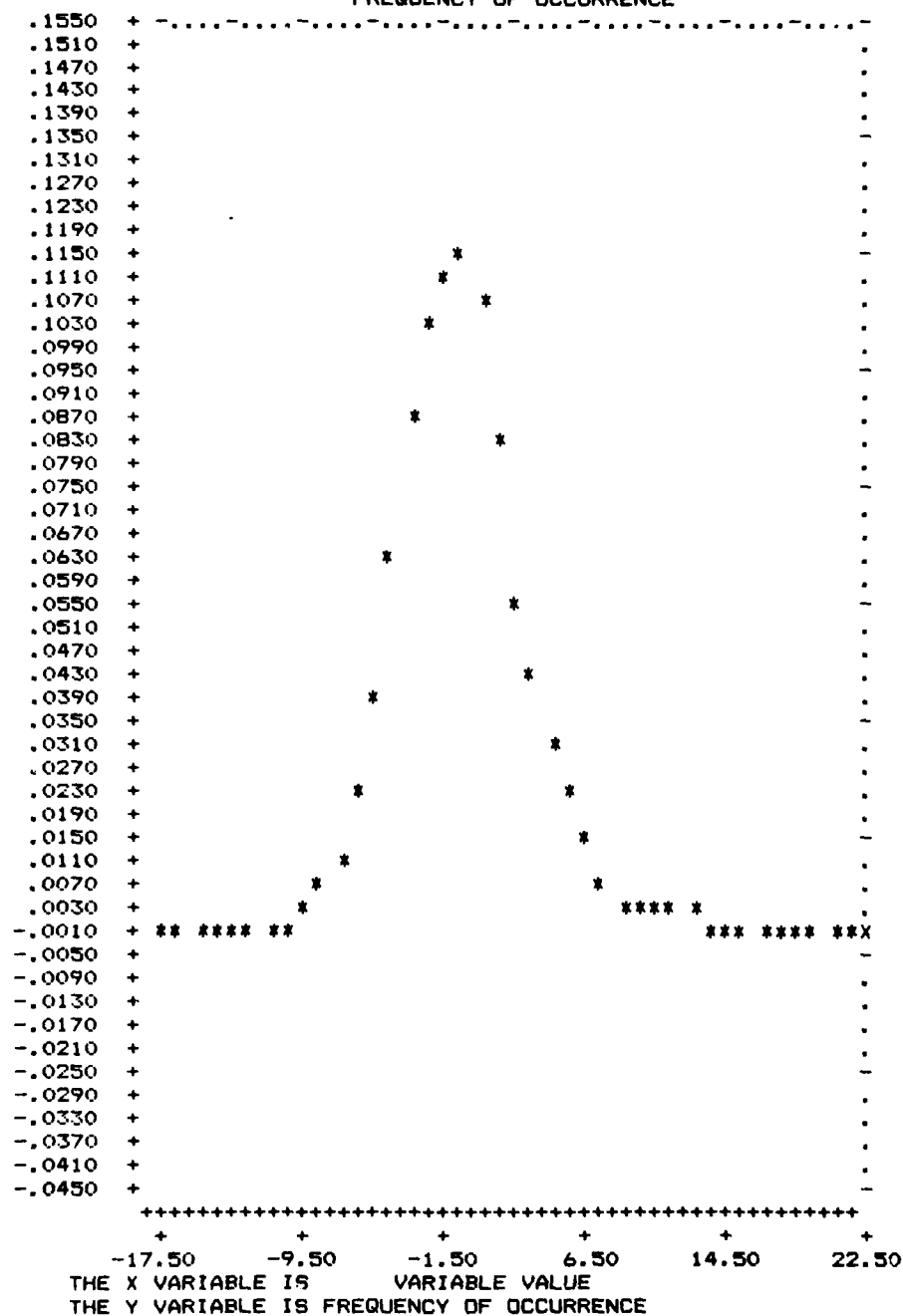
Figure M-3. COMBINED FREQUENCY DISTRIBUTION FOR A-7E LATERAL TOUCHDOWN DATA
