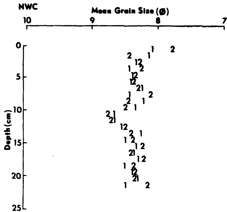
Figure 3. Vertical distribution of sediment mean grain size ( \phi ) measured from cores collected at the NWC site.
