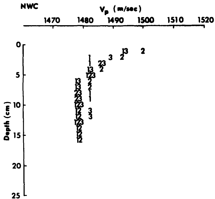
Figure 7. Vertical distribution of sediment compressional wave velocity (m/sec), measured with USI-103 sediment velocimeter, for three (5.8 cm inside diameter) core samples collected at the NWC site.
