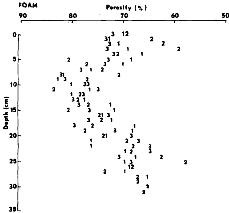
Figure 6. Vertical distribution of sediment porosity (%) measured from cores collected at the FOAM site.
