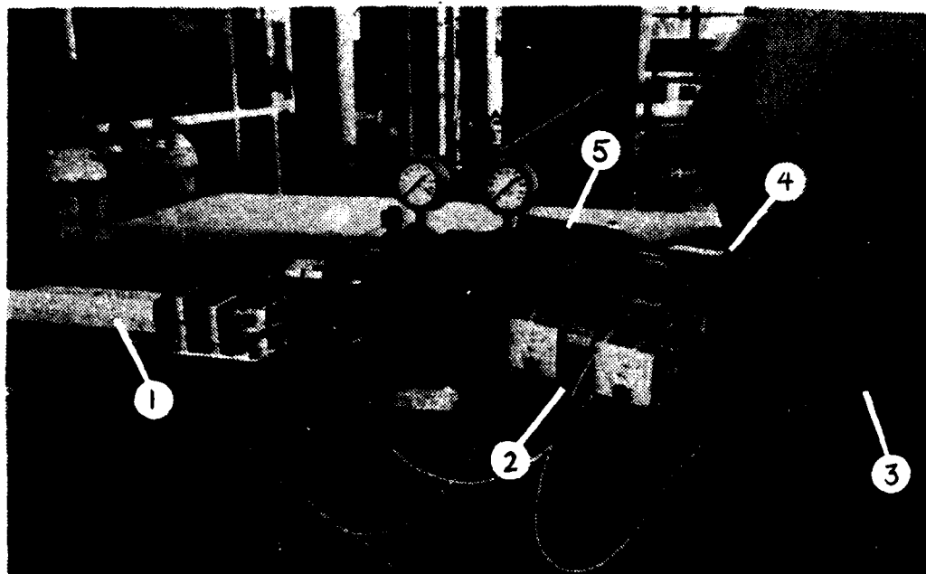
Items indicated are: (1) laser, (2) electrical motor power supply, (3) proximity-sensor amplifier, (4) timer, (5) counter.
