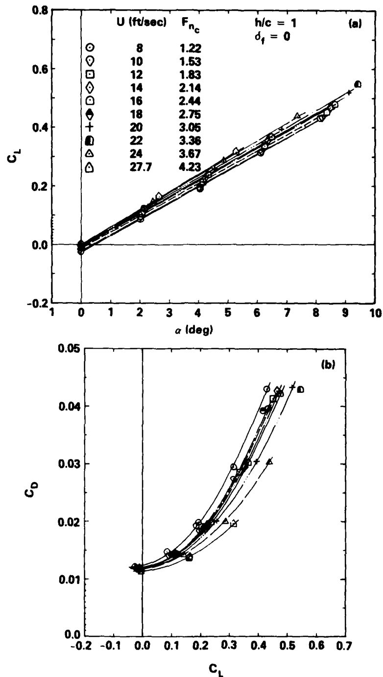
Figure 11 - Measured Hydrofoil Lift and Drag Coefficients for Submergence Ratio h/c = 1 , Zero Flap, Contours of Speed
