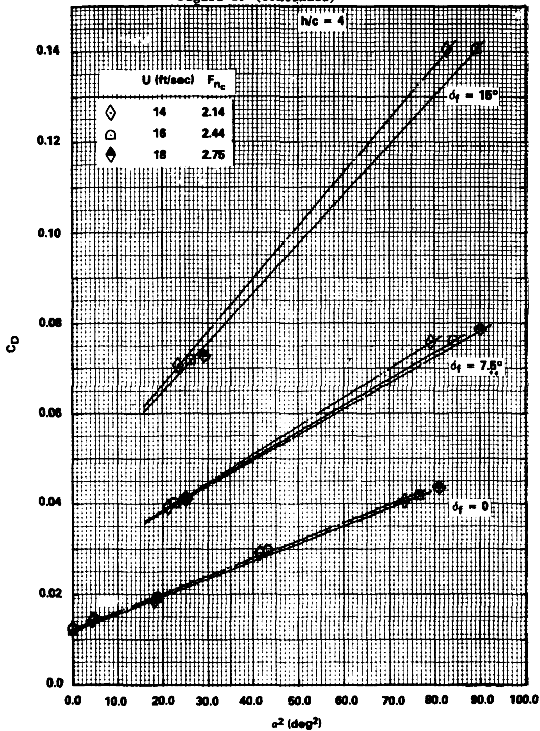
Figure 25b - F_{nc} = 2.14, 2.44, \text{ and } 2.75
