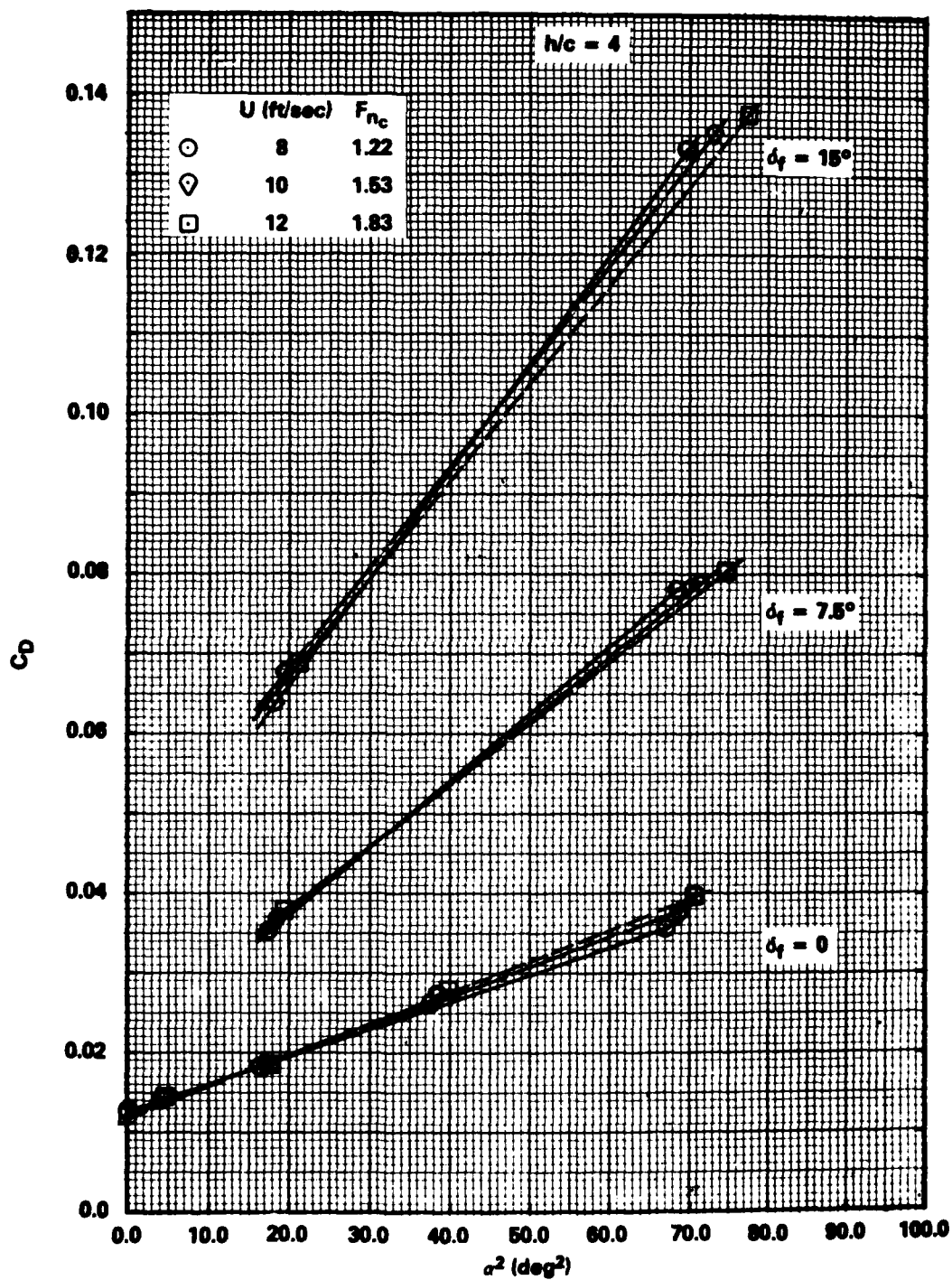
Figure 25a - F_{nc} = 1.22, 1.53 and 1.83
