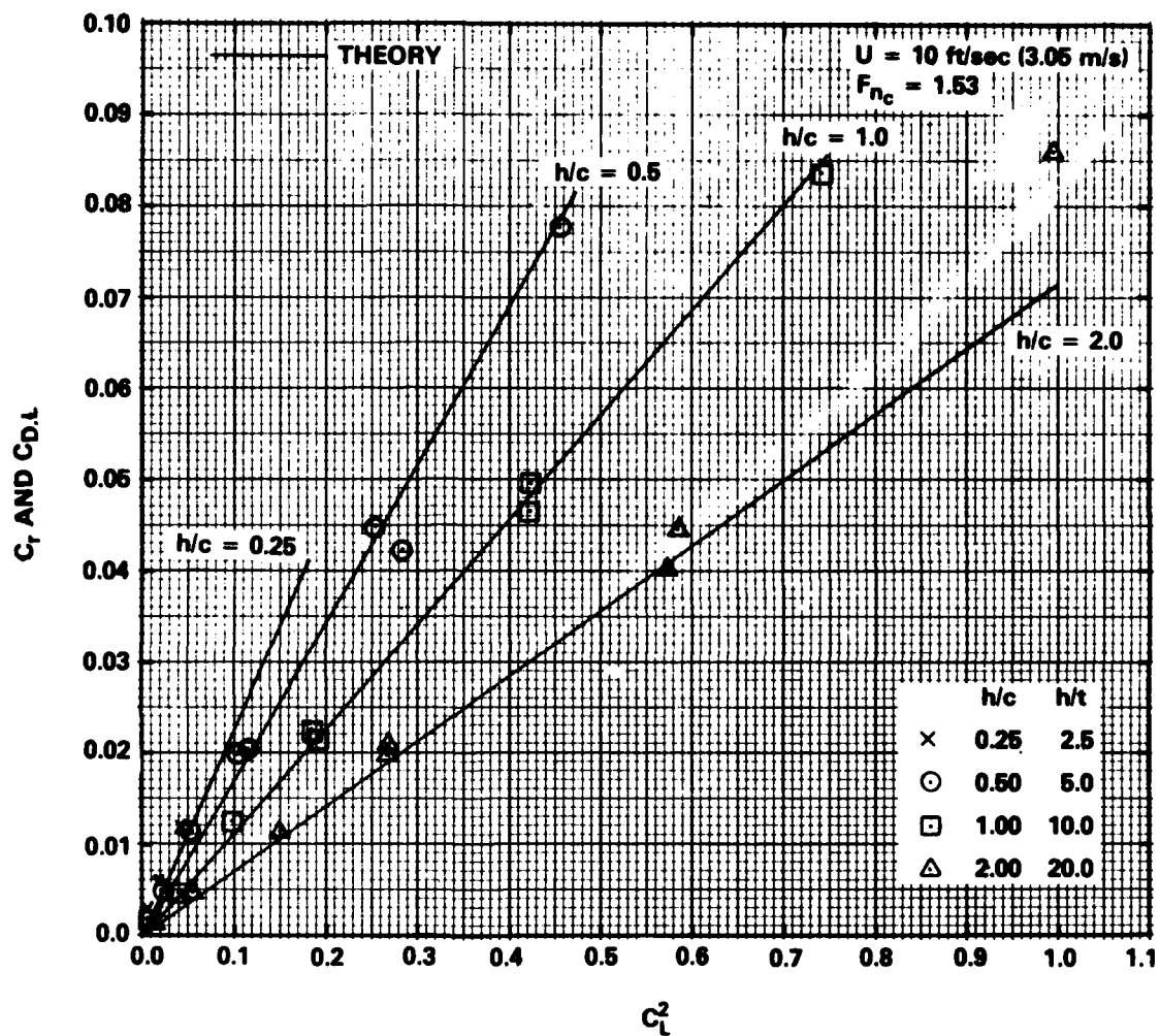
Figure 38 - Comparison of Measured C_r with Calculated C_{D,L} from Lifting Line Theory versus C_L^2 , for F_{nc} = 1.53
