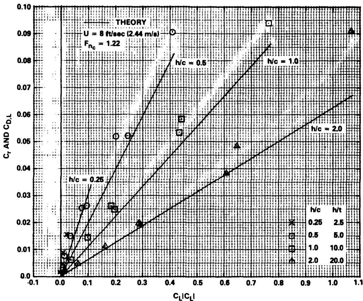
Figure 37 - Comparison of Measured C_r with Calculated C_{D,L} from Lifting Line Theory versus C_L^2/C_L , for F_{nc} = 1.22
