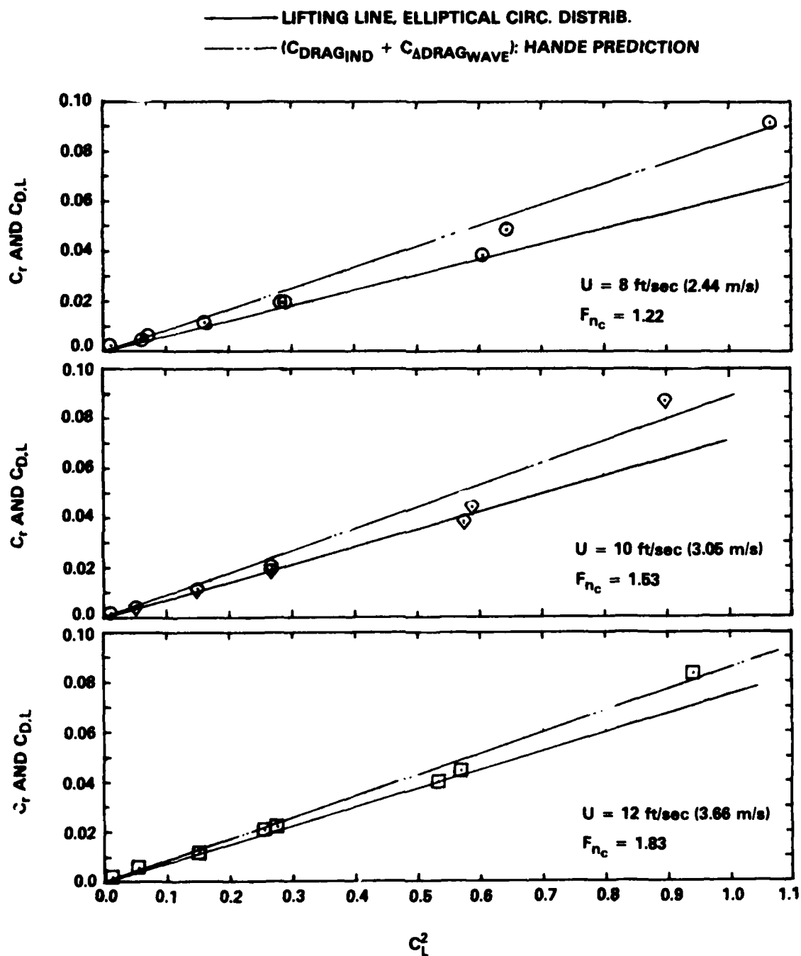
Figure 45 - Comparison of Measured C_r with Predictions of C_{D,L} versus C_L^2 , for Submergence Ratio h/c \approx 2
