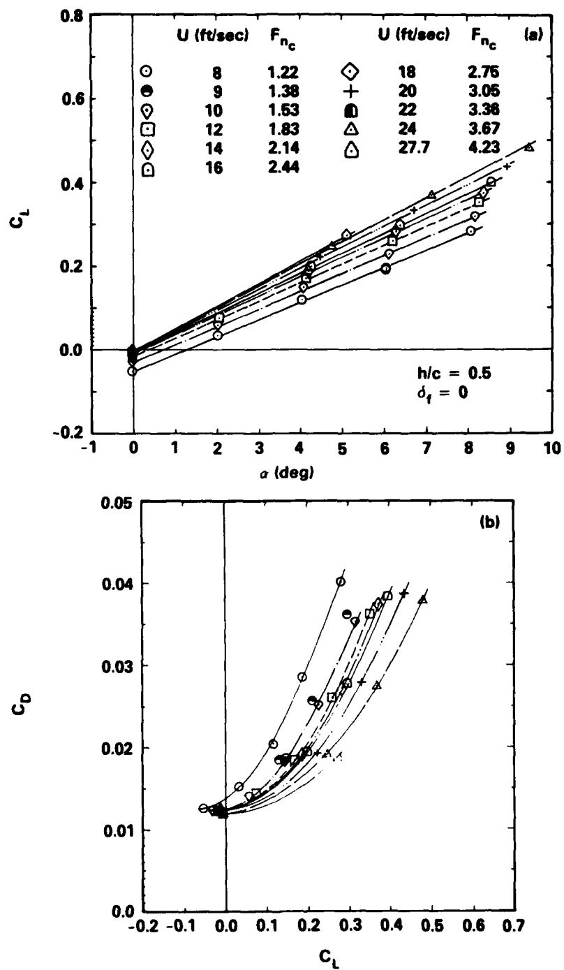
Figure 13 - Measured Hydrofoil Lift and Drag Coefficients for Submergence Ratio h/c = 0.5 , Zero Flap, Contours of Speed
