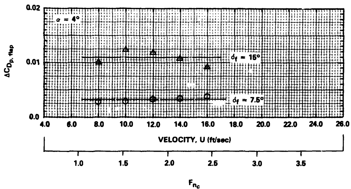
Figure 32 - Inferred Incremental Profile Drag Coefficient due to Flap Deflection versus Speed
