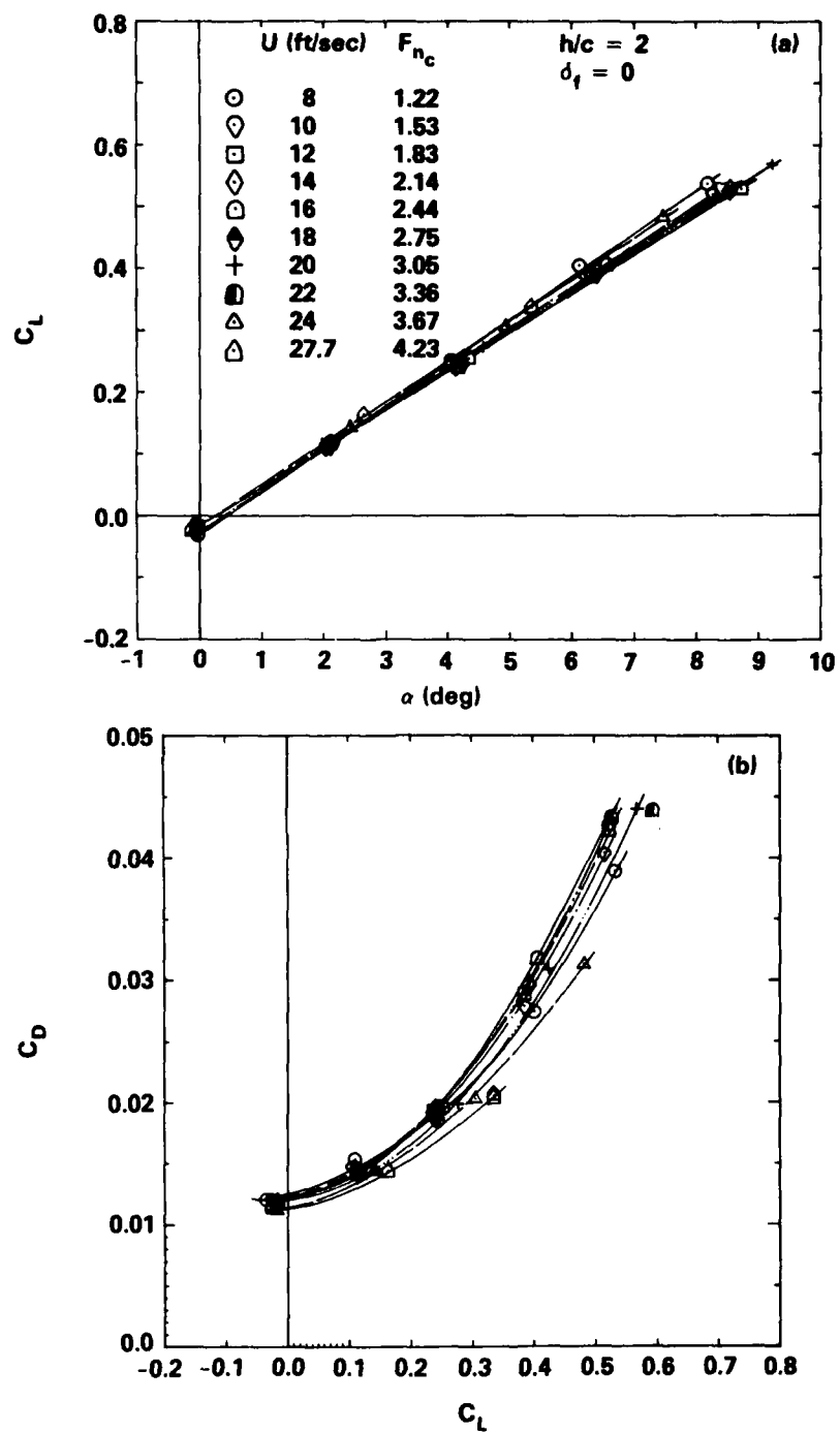
Figure 9 - Measured Hydrofoil Lift and Drag Coefficients for Submergence Ratio h/c = 2 , Zero Flap, Contours of Speed
