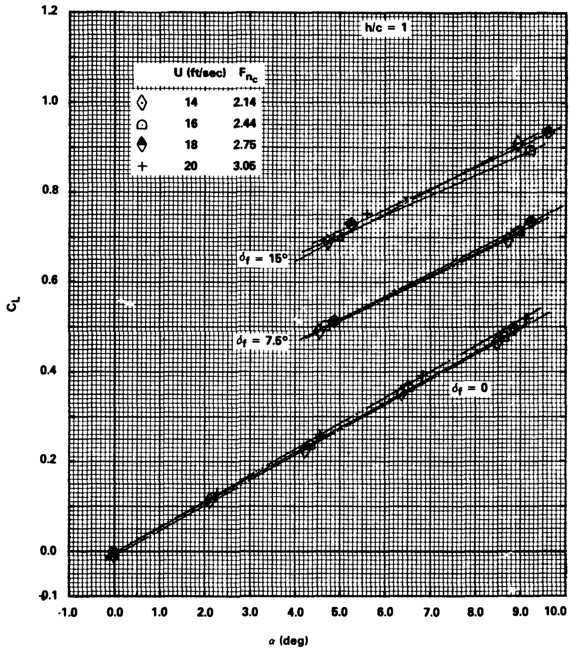
Figure 21b - F_{nc} = 2.14, 2.44, 2.75, \text{ and } 3.05
