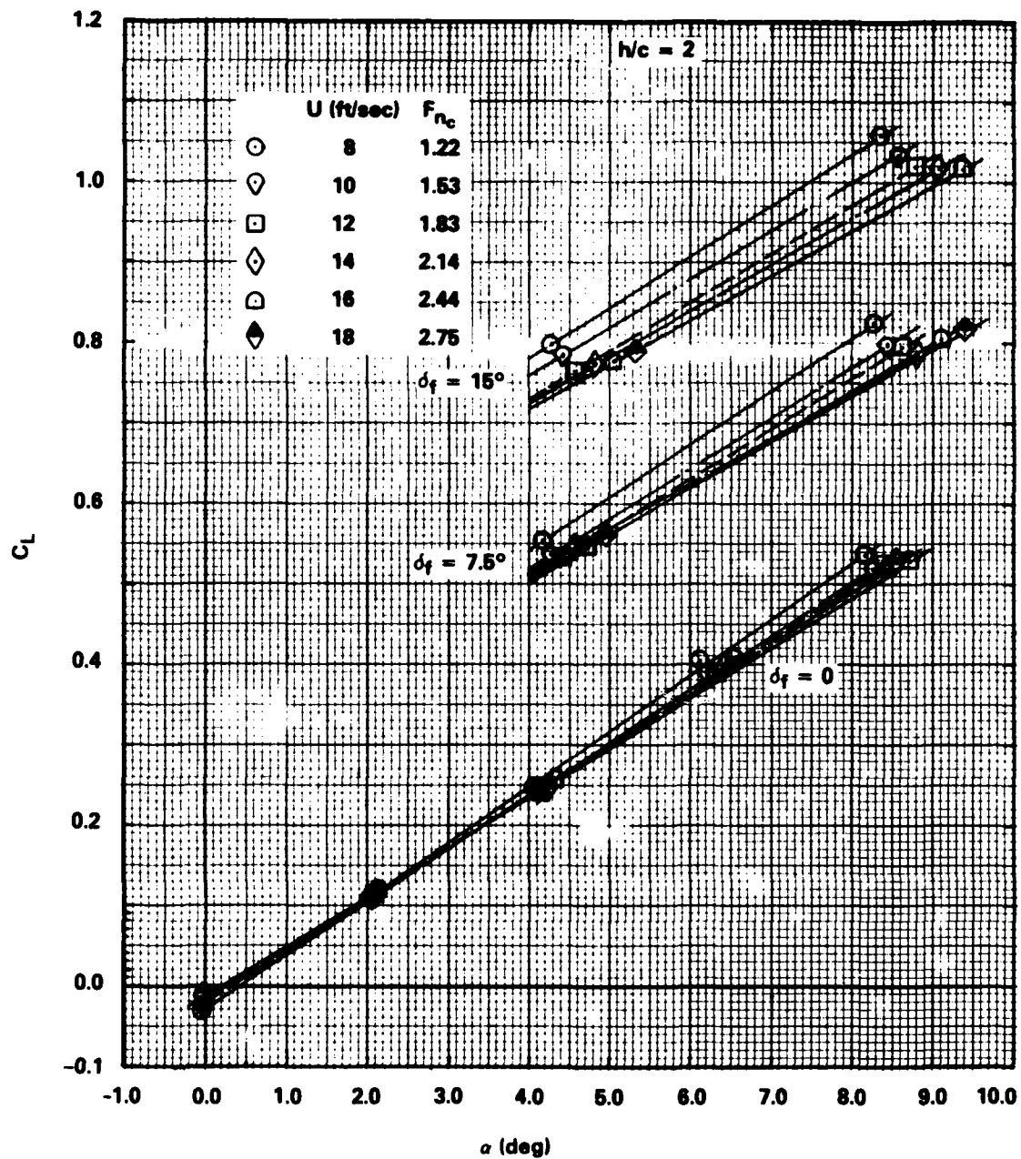
Figure 20 - Effect of Flap Deflection on Lift Coefficient versus Angle of Attack for Submergence Ratio h/c = 2
