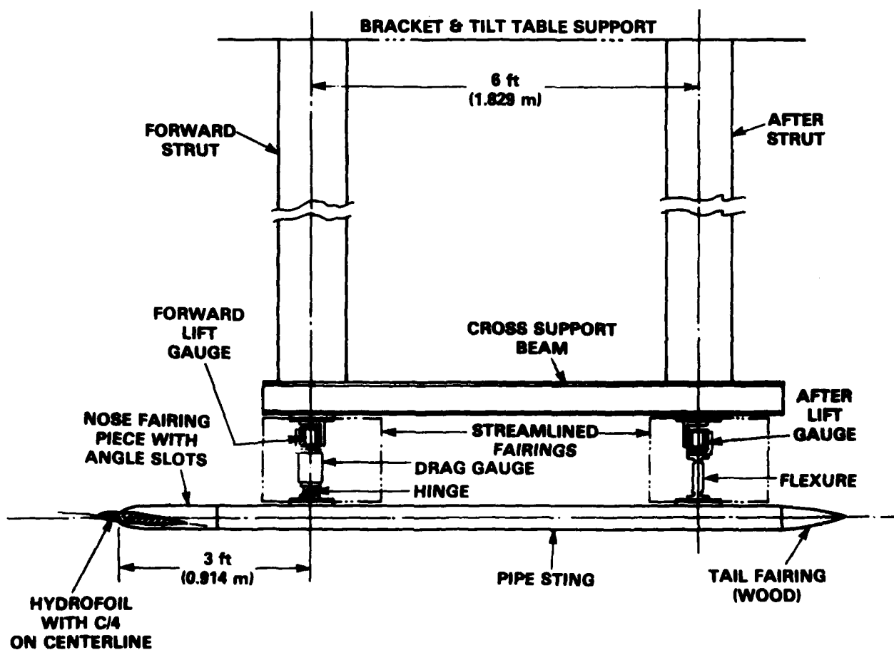
Figure 3 - Sketch of Hydrofoil Forward-Leading Sting and Dynamometer Support System
