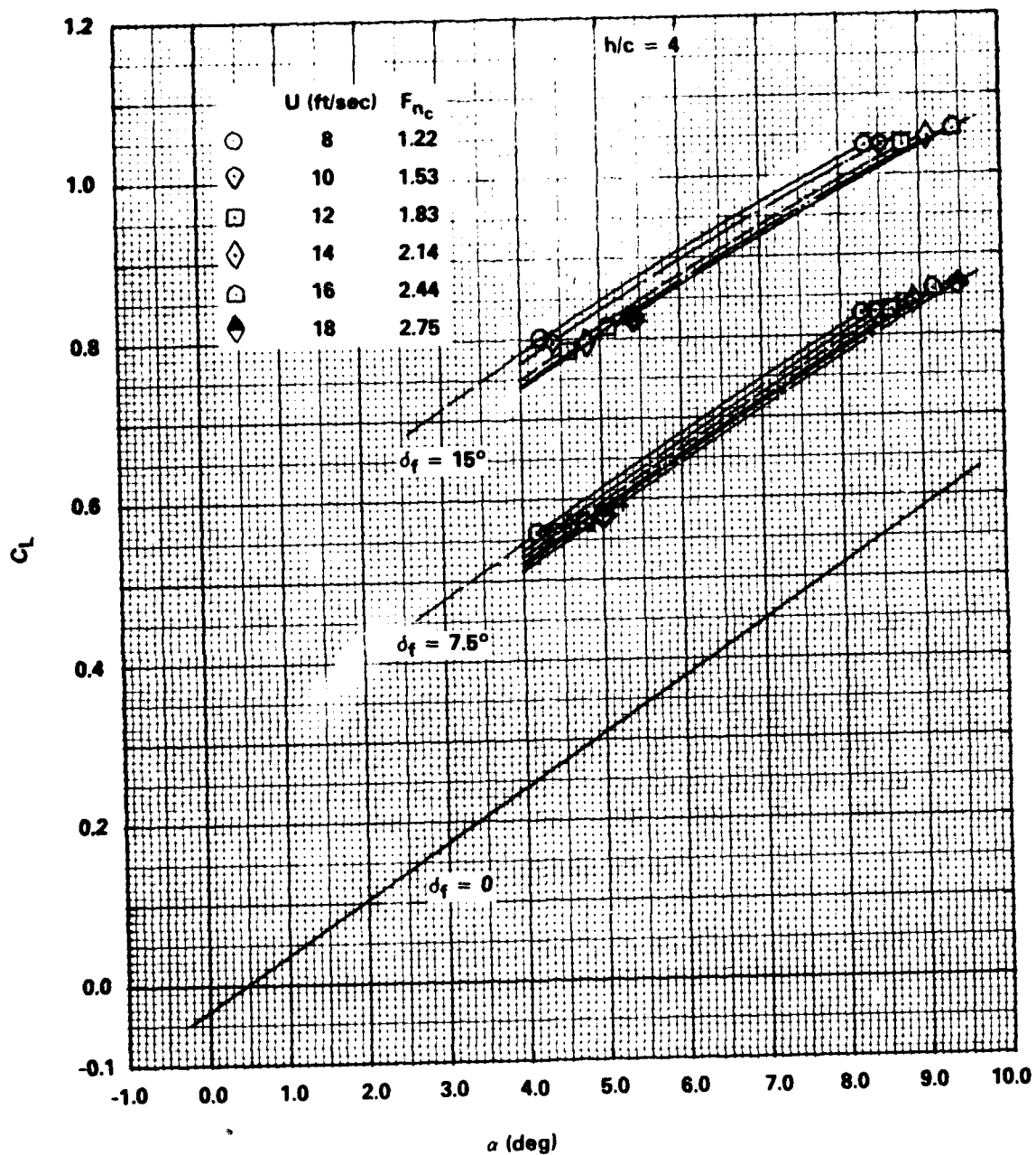
Figure 19 - Effect of Flap Deflection on Lift Coefficient versus Angle of Attack for Submergence Ratio h/c = 4
