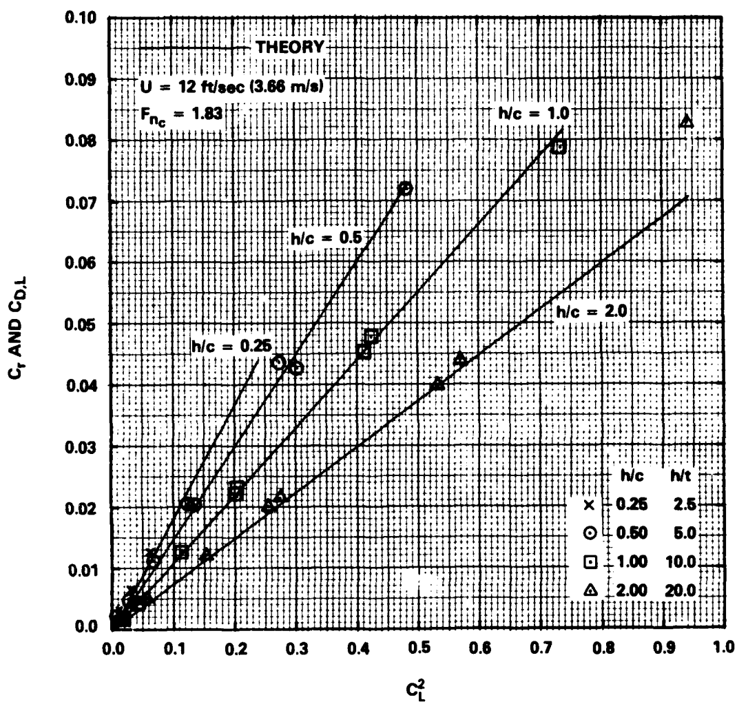
Figure 39 - Comparison of Measured C_L with Calculated C_{D,L} from Lifting Line Theory versus C_L^2 , for F_{nc} = 1.83
