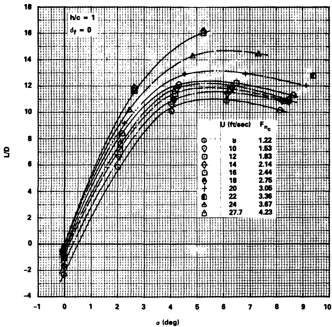
Figure 12 - Hydrofoil Lift-to-Drag Ratio versus Angle of Attack for Submergence Ratio h/c = 1 , Contours of Speed
