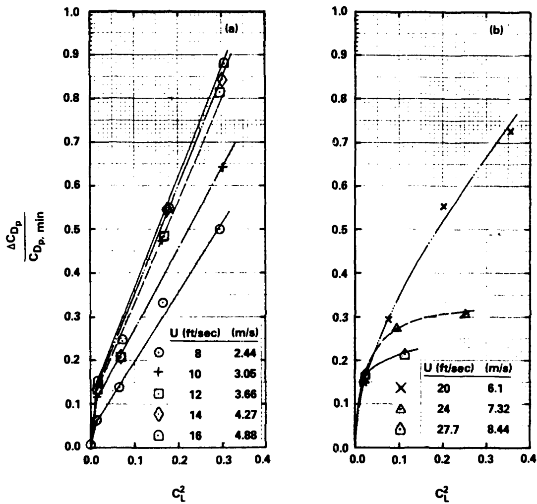
Figure 31 - Inferred Incremental Profile Drag Ratio versus C_L^2 , Contours of Speed
