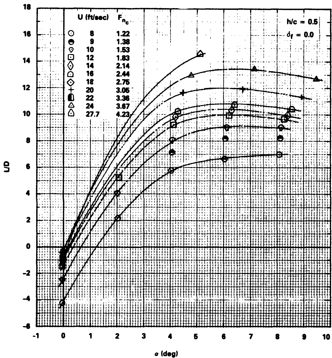
Figure 14 - Hydrofoil Lift-to-Drag Ratio versus Angle of Attack for Submergence Ratio h/c = 0.5 , Contours of Speed
