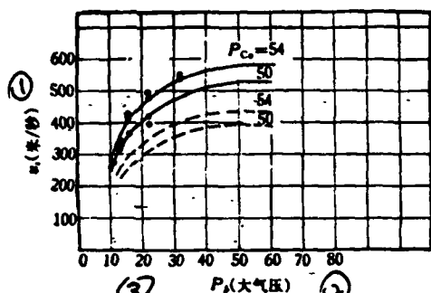
Figure 5. The relation between diaphragm breaking pressure and exit velocity 1-- u_s (m/sec); 2-- P_b (atm) 3--- m_s = 8 g; 4-- m_s = 16 g. Experimental results of this work
