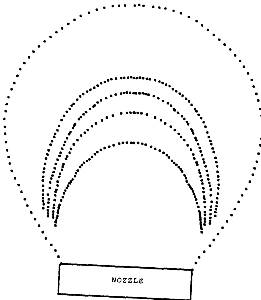
Figure 12 Photochromic Dye Traces in Growing Droplet
