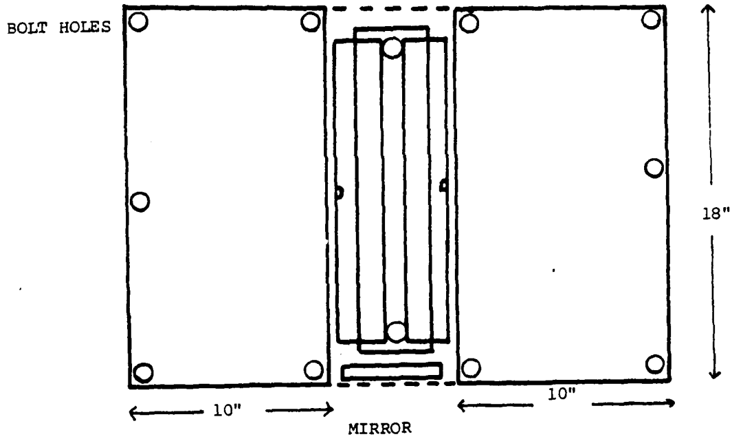
Figure 7 Final Assembly
