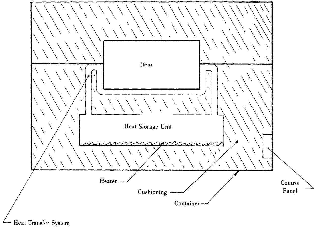
Figure 12-5. Schematic Drawing of a Container Using Thermophormic Materials for Temperature Control
