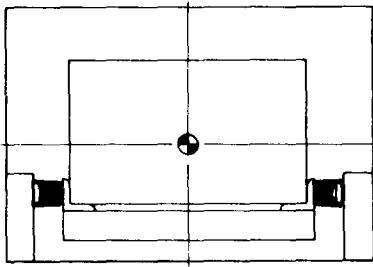
Figure 6-5. Lateral View of Typical Suspension System
