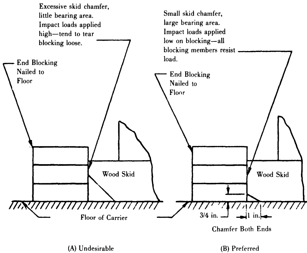
Figure 9-10. Skid Chamfers
