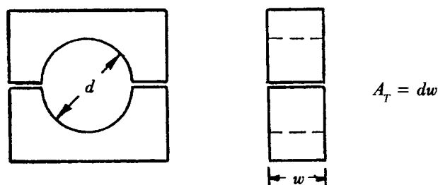
Figure 7-34. Effective Bearing Area of Semicircular Yoke Supports
