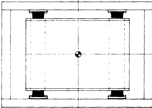
Figure 6-6. Plan View of Typical Suspension System
