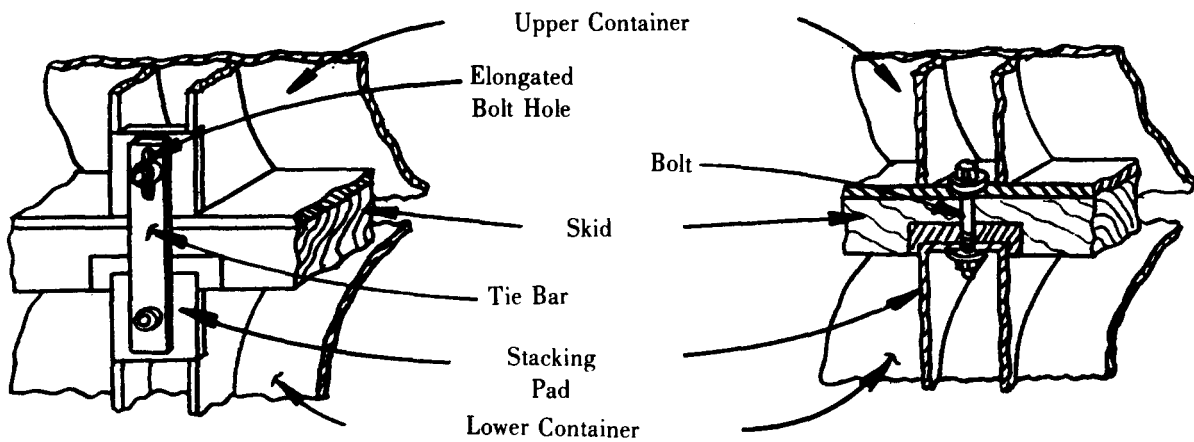
Figure 9-9. Unitizing Devices
