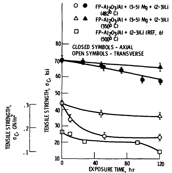
Figure 6. - Effect of isothermal exposure on room temperature axial and transverse tensile strengths of 55 vol % FP- \text{Al}_2\text{O}_3/\text{aluminum} composites as a function of exposure time.
