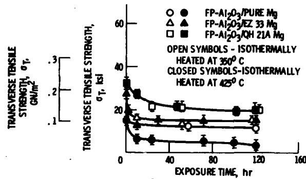
Figure 15. - Effect of thermal exposure on room temperature transverse tensile strength of 55 vol % FP-Al 2 O 3 /magnesium composites as a function of exposure time.
