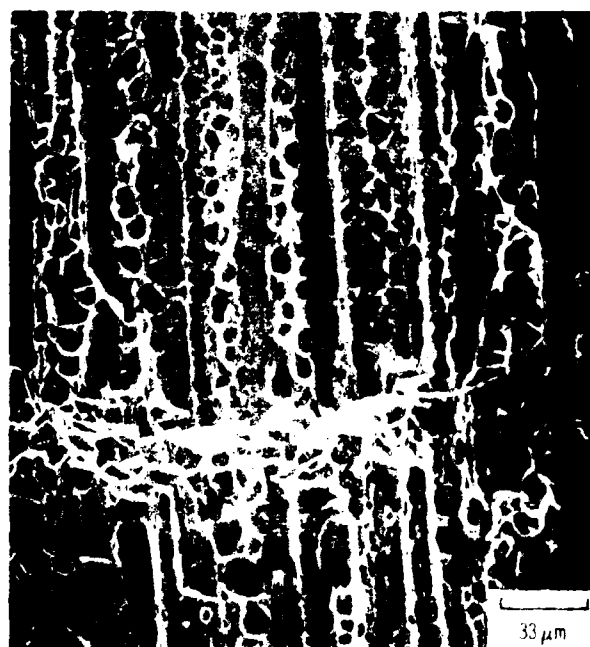
(c) ISOTHERMALLY HEATED AT 472°C FOR 52 HOURS.
