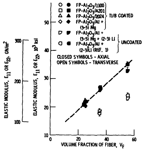
Figure 1 - Axial and transverse elastic moduli of FP- \text{Al}_2\text{O}_3 /aluminum composite as a function of fiber content.
