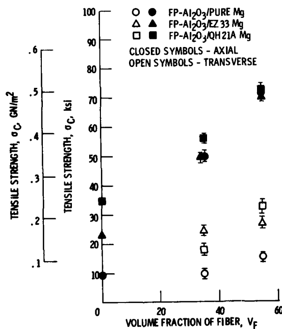
Figure 12. - Axial and transverse tensile strengths of FP-Al 2 O 3 /magnesium composites as a function of fiber content.
