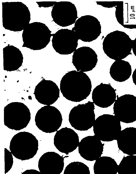
Figure 3. - Photomicrograph of as-received 55 vol % FP-Al 2 O 3 /Al-(2-3) Li-(3-5)Mg specimen.
