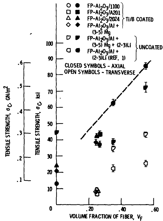
Figure 2 - Axial and transverse tensile strength of FP- \text{Al}_2\text{O}_3 /aluminum composites as a function of fiber content.
