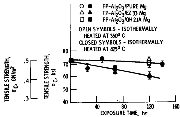
Figure 14. - Effect of thermal exposure on room temperature axial tensile strength of 55 vol % FP- \text{Al}_2\text{O}_3 /magnesium composites as a function of exposure time.
