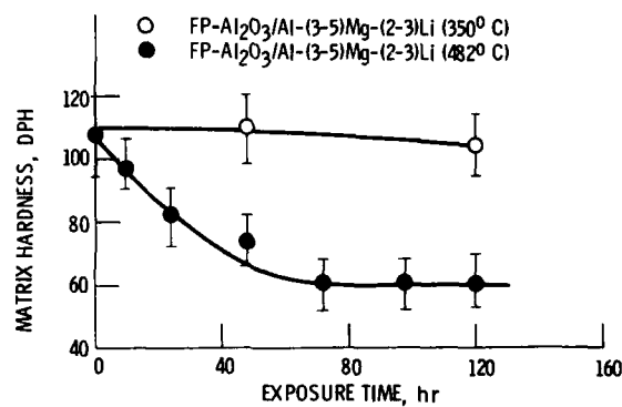
Figure 7. - Effect of isothermal exposure on room temperature matrix hardness of 55 vol % FP- \text{Al}_2\text{O}_3/\text{Al} -(3-5)Mg-(2-3)Li as a function of exposure time.
