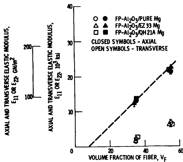
Figure 11. - Axial and transverse elastic moduli of FP-Al 2 O 3 /magnesium composites as a function of fiber content.
