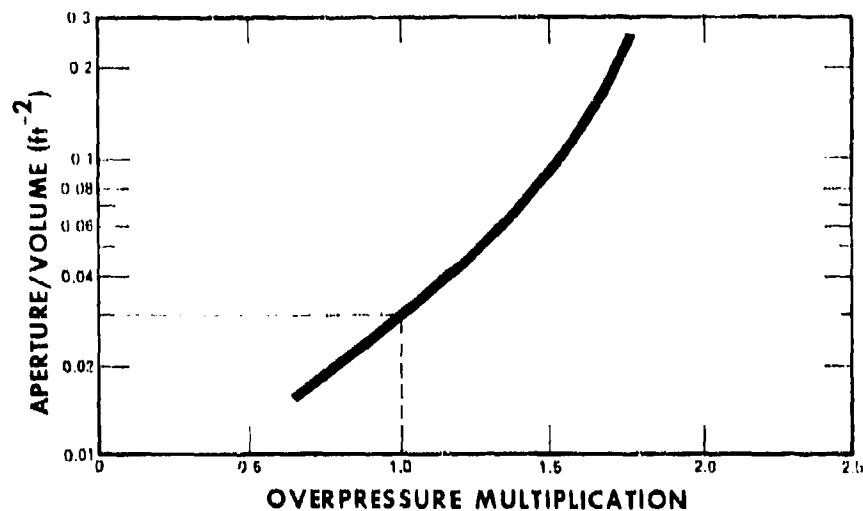
FIGURE 10. OVERPRESSURE MULTIPLICATION PLOTTED AS A FUNCTION OF OPENING/VOLUME RATIO.
