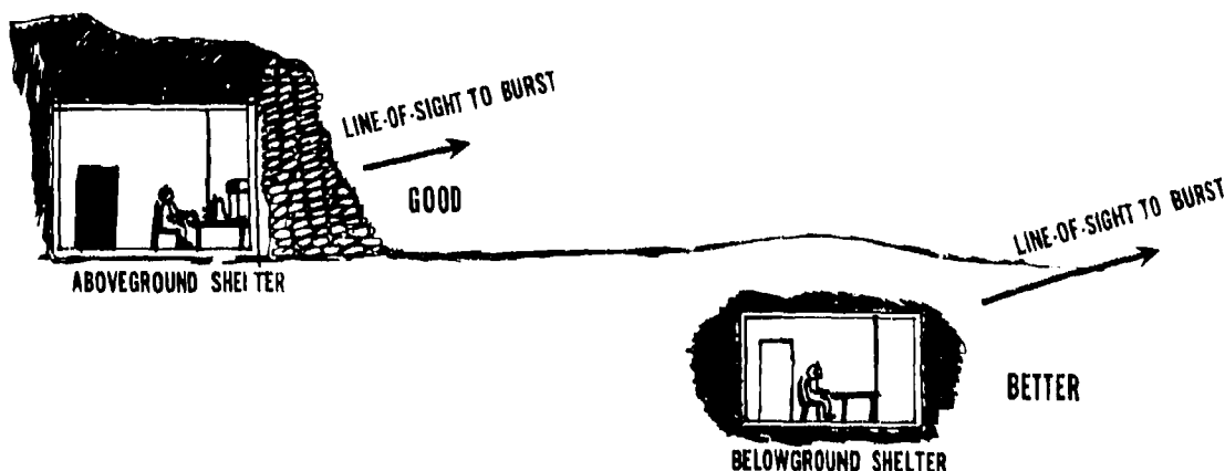
FIGURE 8. SECTION VIEWS OF SHELTERS.
