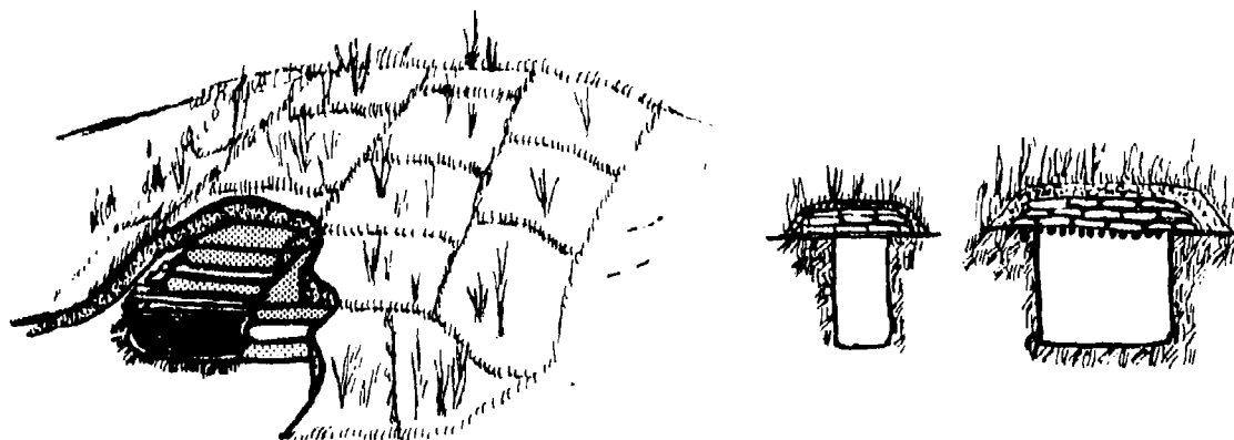
FIGURE 9. PROTECTING SANDBAGS WITH SOD AND EARTH COVER.
