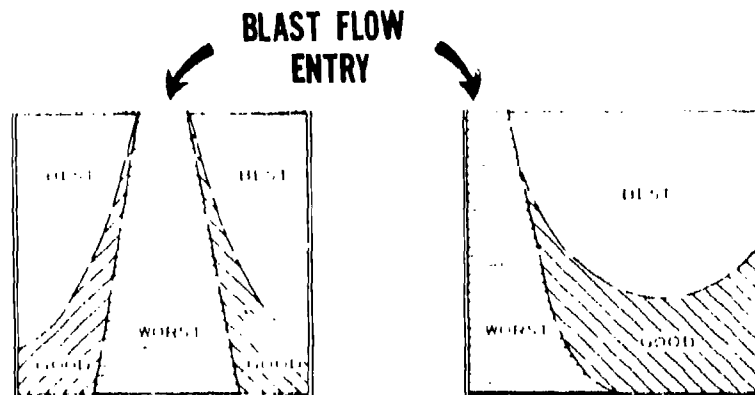
6. PERSONNEL PLACEMENT ZONES FOR VARIOUS LEVELS OF PROTECTION
