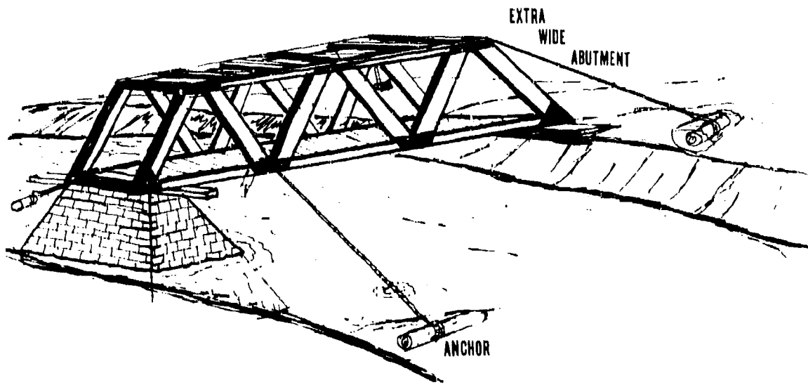
FIGURE 27. PROTECTING BRIDGES.
