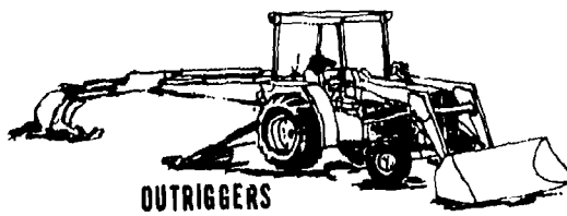
FIGURE 17a. ANCHORS, TIEDOWNS, AND OUTRIGGERS.
