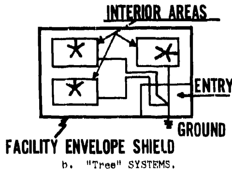
FIGURE 26. GROUNDING CONFIGURATIONS.
