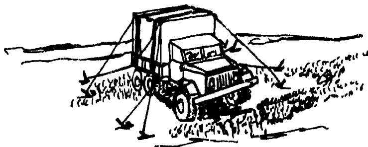
FIGURE 21. ANCHOR AND TIE DOWN VEHICLE AND CARGO.
