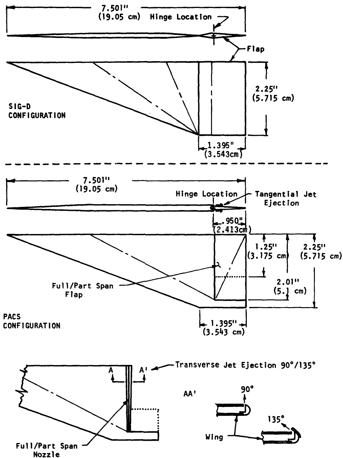
FIGURE 3-6 SIG-D AND PACS HSWT FIN MODELS
