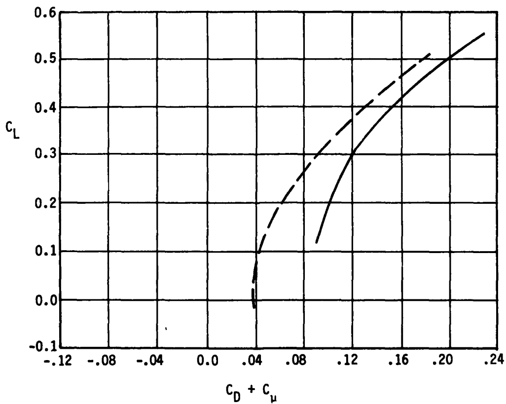
FIGURE 4-7 EFFECT OF JET ANGLE ON LIFT AND DRAG PERFORMANCE - PACS-2
